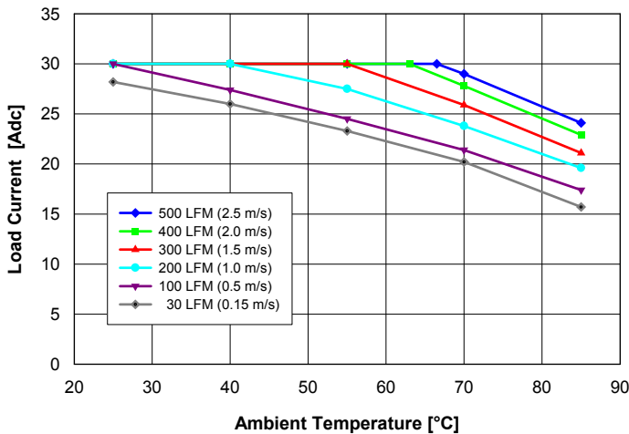
Fig. 1: Available load current vs. ambient air temperature and air-flow rates for Q48S30033 converter mounted vertically with air flowing from pin 3 to pin 1, MOSFET temperature \leq 120^{\circ}\text{C} , V_{in} = 54\text{ V} .
