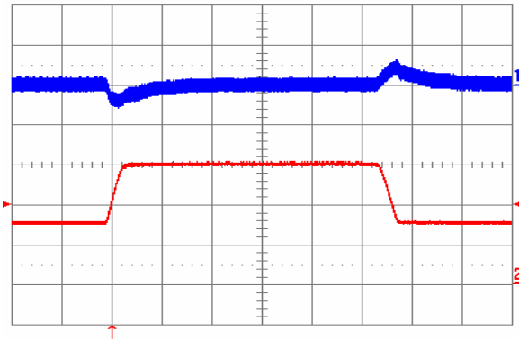
Fig. 20: Output voltage response to load current step-change (7.5 A – 15 A – 7.5 A) at V_{in} = 48 V. Top trace: output voltage (100 mV/div.). Bottom trace: load current (5 A/div.). Current slew rate: 0.1 A/ \mu s. C_o = 1 \mu F ceramic. Time scale: 0.2 ms/div.
