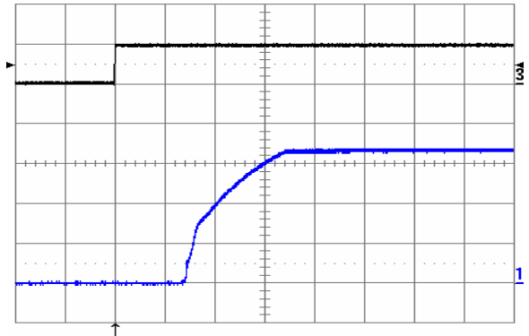
Fig. 19: Turn-on transient at full rated load current (resistive) plus 10,000 \mu F at V_{in} = 48 V, triggered via ON/OFF pin. Top trace: ON/OFF signal (5 V/div.). Bottom trace: output voltage (1 V/div.). Time scale: 1 ms/div.
