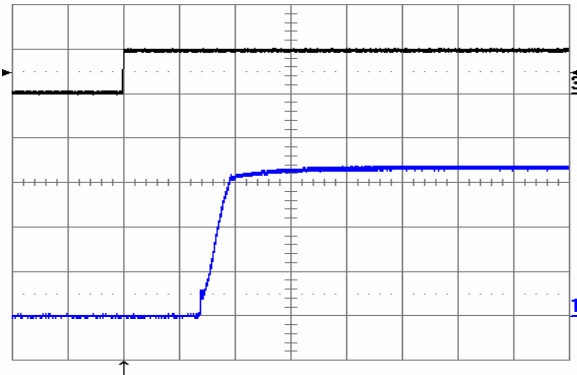
Fig. 18: Turn-on transient at full rated load current (resistive) with no output capacitor at V_{in} = 48 V, triggered via ON/OFF pin. Top trace: ON/OFF signal (5 V/div.). Bottom trace: output voltage (1 V/div.) Time scale: 1 ms/div.
