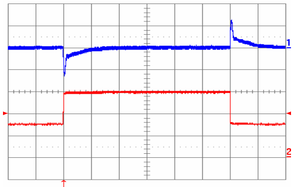
Fig. 21: Output voltage response to load current step-change (7.5 A – 15 A – 7.5 A) at V_{in} = 48 V. Top trace: output voltage (100 mV/div.). Bottom trace: load current (5 A/div.). Current slew rate: 5 A/ \mu s. C_o = 450 \mu F tantalum + 1 \mu F ceramic. Time scale: 0.2 ms/div.
