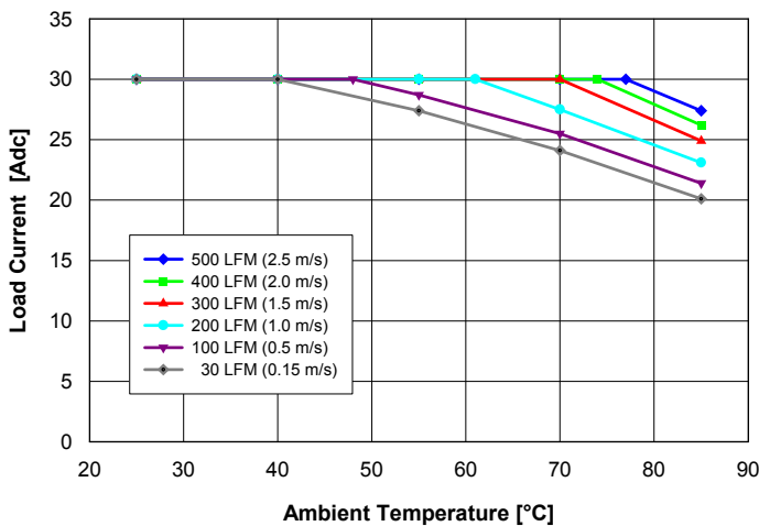
Fig. 1: Available load current vs. ambient air temperature and air-flow rates for Q48S30020 converter mounted vertically with air flowing from pin 3 to pin 1, MOSFET temperature \leq 120^{\circ}\text{C} , V_{in} = 54\text{ V} .
