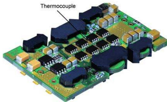
Fig. 28: Location of the thermocouple for thermal testing.
