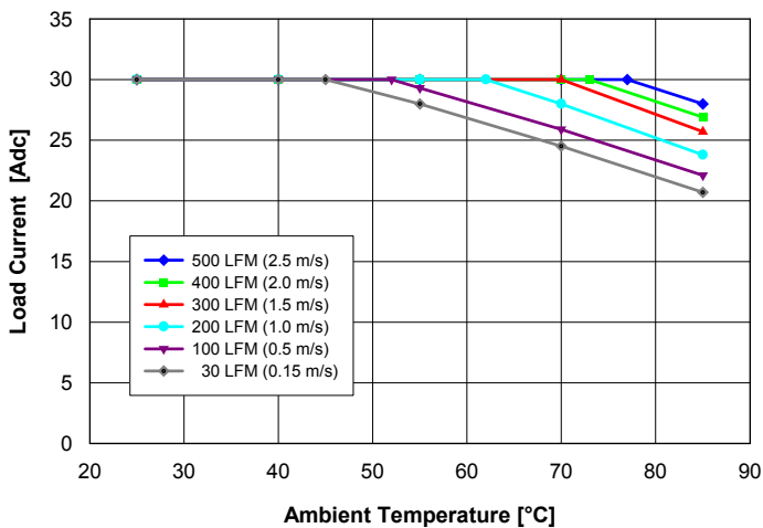
Fig. 1: Available load current vs. ambient air temperature and air-flow rates for Q48S30018 converter mounted vertically with air flowing from pin 3 to pin 1, MOSFET temperature \leq 120^{\circ}\text{C} , V_{in} = 54\text{ V} .
