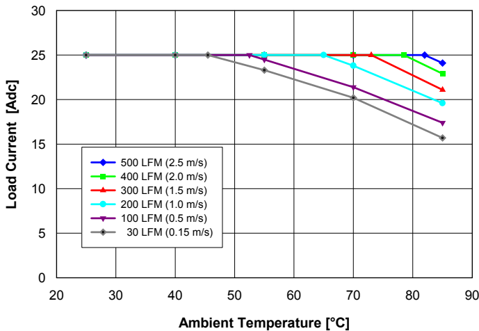
Fig. 1: Available load current vs. ambient air temperature and air-flow rates for Q48S25033 converter mounted vertically with air flowing from pin 3 to pin 1, MOSFET temperature \leq 120^{\circ}\text{C} , V_{in} = 54\text{ V} .
