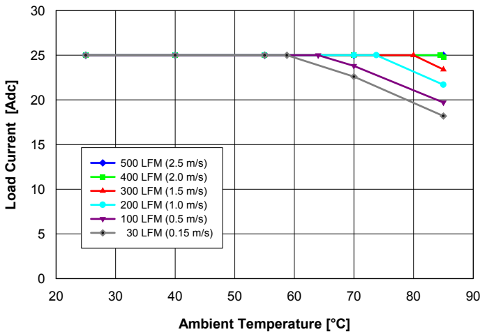
Fig. 1: Available load current vs. ambient air temperature and air-flow rates for Q48S25025 converter mounted vertically with air flowing from pin 3 to pin 1, MOSFET temperature \leq 120^{\circ}\text{C} , V_{in} = 54\text{ V} .
