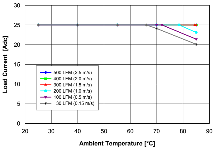
Fig. 1: Available load current vs. ambient air temperature and air-flow rates for Q48S25020 converter mounted vertically with air flowing from pin 3 to pin 1, MOSFET temperature \leq 120^{\circ}\text{C} , V_{in} = 54\text{ V} .
