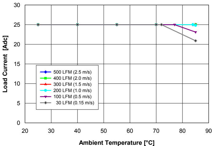
Fig. 1: Available load current vs. ambient air temperature and air-flow rates for Q48S25015 converter mounted vertically with air flowing from pin 3 to pin 1, MOSFET temperature \leq 120^{\circ}\text{C} , V_{in} = 54\text{ V} .
