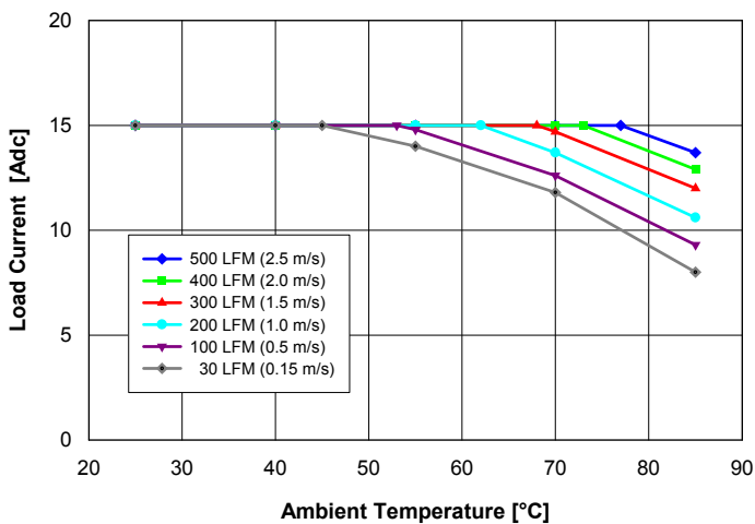
Fig. 1: Available load current vs. ambient air temperature and air-flow rates for Q48S15050 converter mounted vertically with air flowing from pin 3 to pin 1, MOSFET temperature \leq 120^{\circ}\text{C} , V_{in} = 54\text{ V} .
