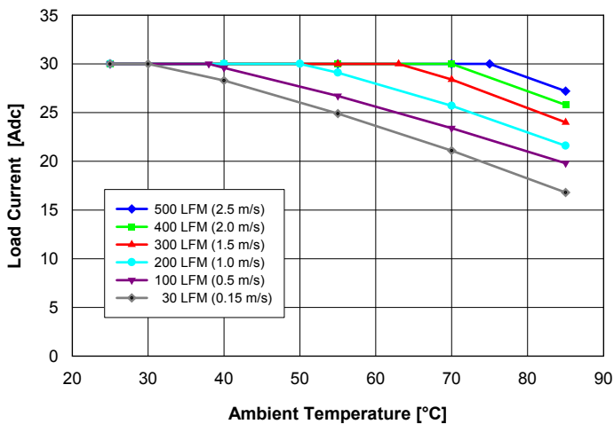
Fig. 1: Available load current vs. ambient air temperature and air-flow rates for Q24T30025 converter mounted vertically with air flowing from pin 3 to pin 1, MOSFET temperature \leq 120^{\circ}\text{C} , V_{in} = 27\text{ V} .
