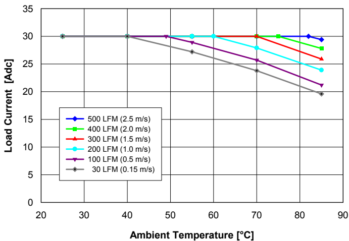
Fig. 1: Available load current vs. ambient air temperature and air-flow rates for Q24T30018 converter mounted vertically with air flowing from pin 3 to pin 1, MOSFET temperature \leq 120^{\circ}\text{C} , V_{in} = 27\text{ V} .
