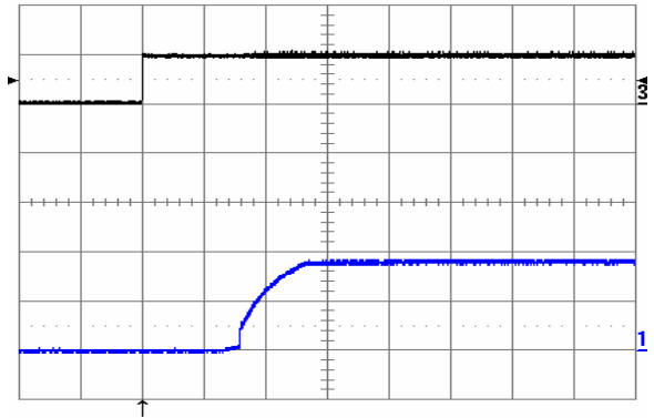
Fig. 19: Turn-on transient at full rated load current (resistive) plus 10,000 \mu F at V_{in} = 24 V, triggered via ON/OFF pin. Top trace: ON/OFF signal (5 V/div.). Bottom trace: output voltage (1 V/div.). Time scale: 1 ms/div.
