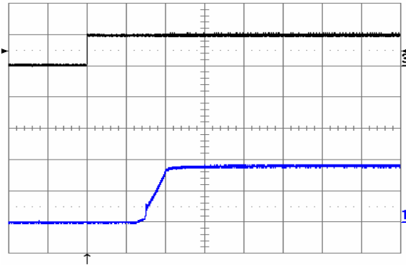
Fig. 18: Turn-on transient at full rated load current (resistive) with no output capacitor at V_{in} = 24 V, triggered via ON/OFF pin. Top trace: ON/OFF signal (5 V/div.). Bottom trace: output voltage (1 V/div.) Time scale: 1 ms/div.
