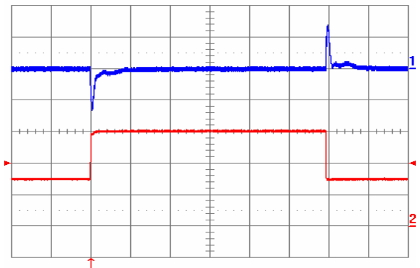
Fig. 21: Output voltage response to load current step-change (7.5 A – 15 A – 7.5 A) at V_{in} = 24 V. Top trace: output voltage (100 mV/div.). Bottom trace: load current (5 A/div.). Current slew rate: 5 A/ \mu s. C_o = 450 \mu F tantalum + 1 \mu F ceramic. Time scale: 0.2 ms/div.
