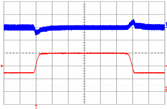
Fig. 20: Output voltage response to load current step-change (7.5 A – 15 A – 7.5 A) at V_{in} = 24 V. Top trace: output voltage (100 mV/div.). Bottom trace: load current (5 A/div.). Current slew rate: 0.1 A/ \mu s. C_o = 1 \mu F ceramic. Time scale: 0.2 ms/div.
