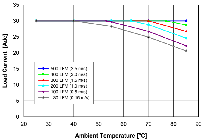
Fig. 1: Available load current vs. ambient air temperature and airflow rates for Q24T30015 converter mounted vertically with air flowing from pin 3 to pin 1, MOSFET temperature \leq 120^{\circ}\text{C} , V_{in} = 27\text{ V} .
