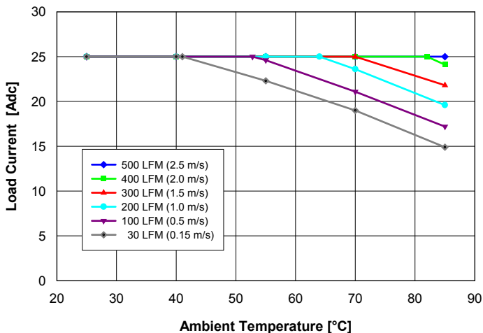
Fig. 1: Available load current vs. ambient air temperature and airflow rates for Q24T25033 converter mounted vertically with air flowing from pin 3 to pin 1, MOSFET temperature \leq 120^{\circ}\text{C} , V_{in} = 27\text{ V} .
