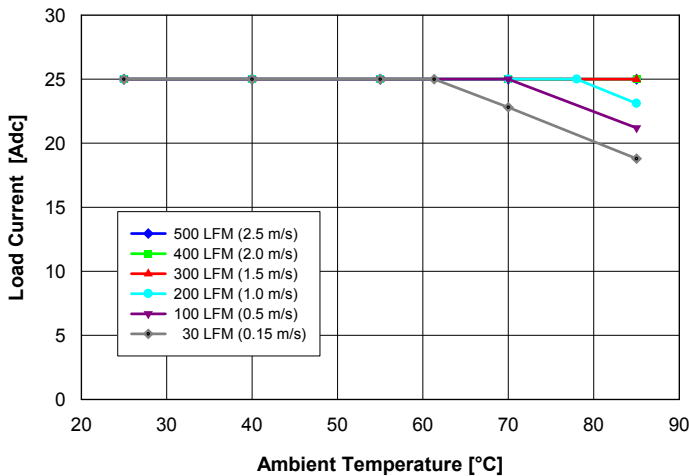
Fig. 1: Available load current vs. ambient air temperature and air flow rates for Q24T25020 converter mounted vertically with air flowing from pin 3 to pin 1, MOSFET temperature \leq 120^{\circ}\text{C} , V_{in} = 27\text{ V} .
