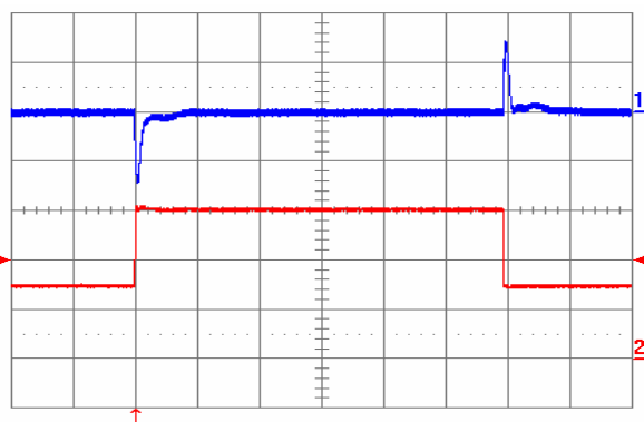
Fig. 21: Output voltage response to load current step-change (7.5 A – 15 A – 7.5 A) at V_{in} = 24\text{ V} . Top trace: output voltage (100 mV/div). Bottom trace: load current (5 A/div). Current slew rate: 5 A/ \mu\text{s} . C_o = 450\ \mu\text{F} tantalum + 1 \mu\text{F} ceramic. Time scale: 0.2 ms/div.
