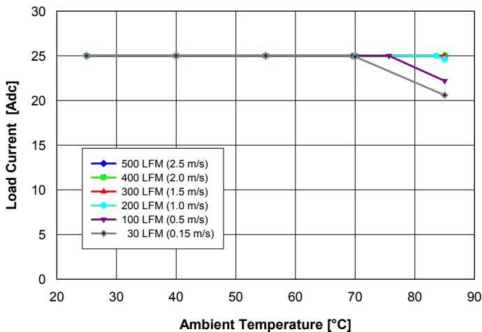
Fig. 1: Available load current vs. ambient air temperature and air-flow rates for Q24T25015 converter mounted vertically with air flowing from pin 3 to pin 1, MOSFET temperature \leq 120^{\circ}\text{C} , V_{in} = 27\text{ V} .
