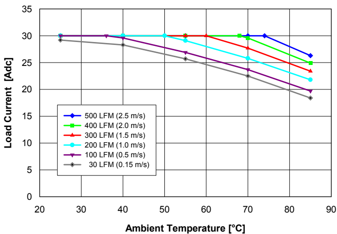
Fig. 1: Available load current vs. ambient air temperature and air-flow rates for Q24S30025 converter mounted vertically with air flowing from pin 3 to pin 1, MOSFET temperature \leq 120^{\circ}\text{C} , V_{in} = 27\text{ V} .
