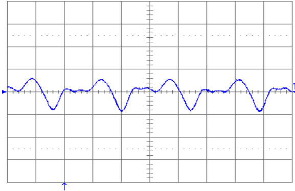
Fig. 22: Output voltage ripple (20 mV/div.) at full rated load current into a resistive load with C_o = 10\ \mu\text{F} tantalum + 1\ \mu\text{F} ceramic and V_{in} = 24\ \text{V} . Time scale: 1\ \mu\text{s}/\text{div} .
