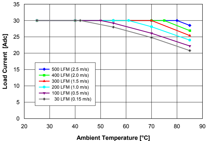
Fig. 1: Available load current vs. ambient air temperature and air-flow rates for Q24S30018 converter mounted vertically with air flowing from pin 3 to pin 1, MOSFET temperature \leq 120^{\circ}\text{C} , V_{in} = 27\text{ V} .
