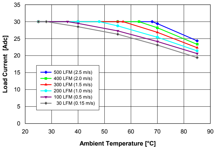
Fig. 12: Available load current vs. ambient temperature and airflow rates for converter mounted horizontally with V_{in} = 27 V, air flowing from pin 3 to pin 4 and maximum FET temperature \leq 120^{\circ}\text{C} .
