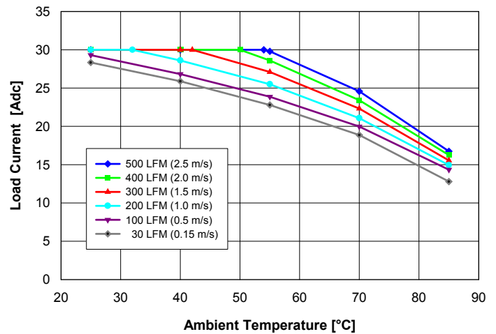
Fig. 13: Available load current vs. ambient temperature and airflow rates for converter mounted horizontally with V_{in} = 27 V, air flowing from pin 3 to pin 4 and maximum FET temperature \leq 105^{\circ}\text{C} .
