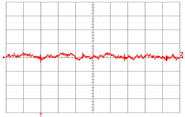
Fig. 25: Input reflected ripple current, i_s (10 mA/div), measured through 10\ \mu\text{H} at the source at full rated load current and V_{in} = 24\ \text{V} . Refer to Fig. 23 for test setup. Time scale: 1\ \mu\text{s}/\text{div} .
