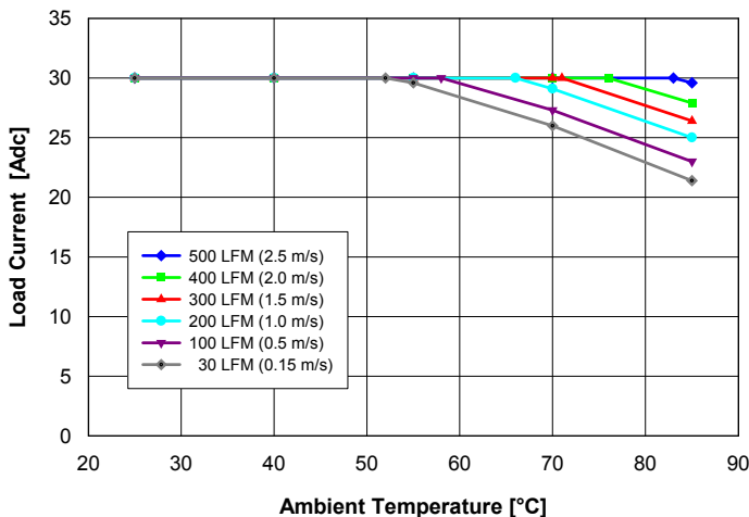
Fig. 1: Available load current vs. ambient air temperature and air-flow rates for Q24S30015 converter mounted vertically with air flowing from pin 3 to pin 1, MOSFET temperature \leq 120^{\circ}\text{C} , V_{in} = 27\text{ V} .
