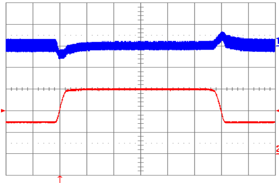
Fig. 20: Output voltage response to load current step-change (7.5 A – 15 A – 7.5 A) at V_{in} = 24\text{ V} . Top trace: output voltage (100 mV/div.). Bottom trace: load current (5 A/div.). Current slew rate: 0.1 A/ \mu\text{s} . C_o = 1\text{ }\mu\text{F} ceramic. Time scale: 0.2 ms/div.
