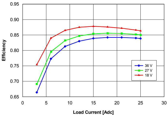
Fig. 16: Efficiency vs. load current and input voltage for converter mounted horizontally with air flowing from pin 3 to pin 4 at a rate of 300 LFM (1.5 m/s) and T_a = 25^\circ\text{C} (MDC10152 Rev.1.0, 16-Mar-10°C).
