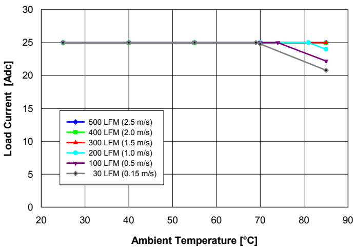
Fig. 1: Available load current vs. ambient air temperature and air-flow rates for Q24S25018 converter mounted vertically with air flowing from pin 3 to pin 1, MOSFET temperature \leq 120^{\circ}\text{C} , V_{in} = 27\text{ V} .
