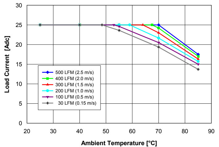
Fig. 13: Available load current vs. ambient temperature and airflow rates for converter mounted horizontally with V_{in} = 27 V, air flowing from pin 3 to pin 4 and maximum FET temperature \leq 105 °C.
