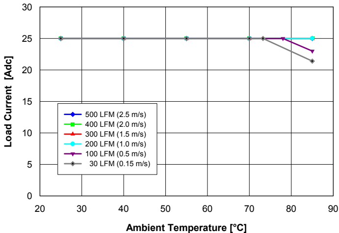
Fig. 1: Available load current vs. ambient air temperature and air-flow rates for Q24S25015 converter mounted vertically with air flowing from pin 3 to pin 1, MOSFET temperature \leq 120^{\circ}\text{C} , V_{in} = 27\text{ V} .
