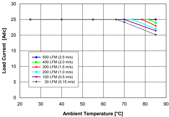
Fig. 12: Available load current vs. ambient temperature and airflow rates for converter mounted horizontally with V_{in} = 27 V, air flowing from pin 3 to pin 4 and maximum FET temperature \leq 120 °C.
