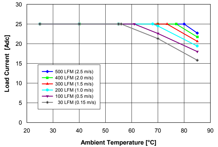
Fig. 11: Available load current vs. ambient air temperature and airflow rates for converter mounted vertically with V_{in} = 27 V, air flowing from pin 3 to pin 1 and maximum FET temperature \leq 105 °C.
