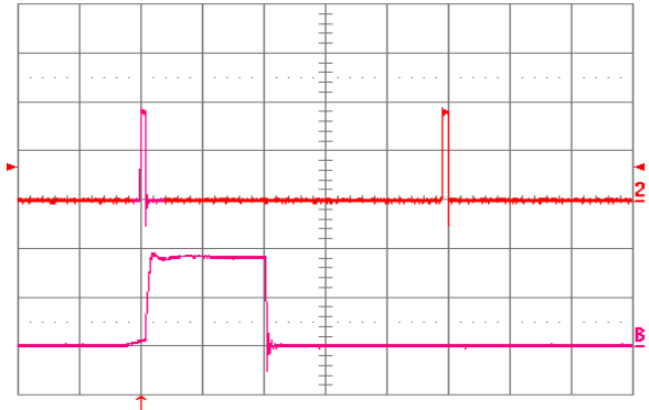
Fig. 27: Load current (top trace, 20 A/div, 20 ms/div) into a 10 mΩ short circuit during restart, at V_{in} = 24 V. Bottom trace (20 A/div, 1 ms/div) is an expansion of the on-time portion of the top trace.
