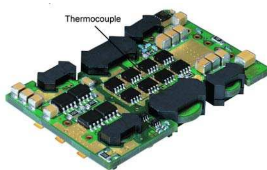
Fig. 28: Location of the thermocouple for thermal testing.
