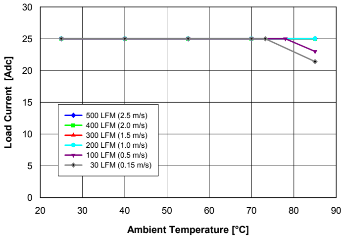
Fig. 10: Available load current vs. ambient air temperature and airflow rates for converter mounted vertically with V_{in} = 27 V, air flowing from pin 3 to pin 1 and maximum FET temperature \leq 120 °C.
