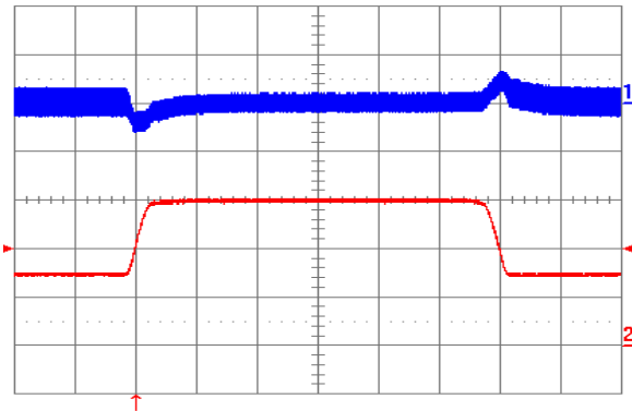
Fig. 20: Output voltage response to load current step-change (7.5 A – 15 A – 7.5 A) at V_{in} = 24\text{ V} . Top trace: output voltage (100 mV/div.). Bottom trace: load current (5 A/div.). Current slew rate: 0.1 A/ \mu\text{s} . C_o = 1\text{ }\mu\text{F} ceramic. Time scale: 0.2 ms/div.
