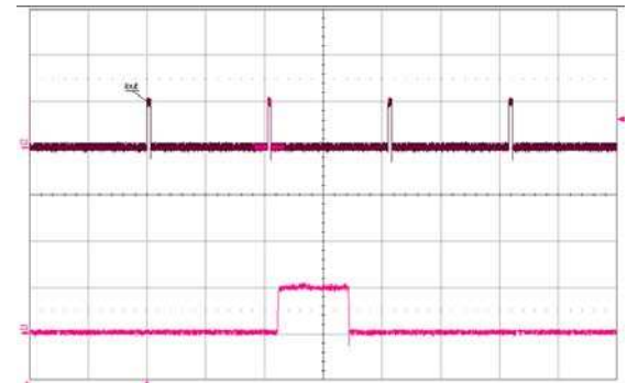
Figure 16. Load current (top trace, 20 A/div., 100 ms/div.) into a 10 m \Omega short circuit during restart, at V_{in} = 48 V. Bottom trace (20 A/div., 5 ms/div.) is an expansion of the on-time portion of the top trace.
