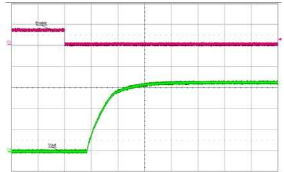
Figure 9. Turn-on waveform at full rated load current (resistive) with 7,500 \mu\text{F} output capacitor at V_{in}=48\text{V} , triggered via ON/OFF pin. Top trace: ON/OFF signal (5V/div.). Bottom trace: Output voltage (1V/div.). Time scale: 2 ms/div.
