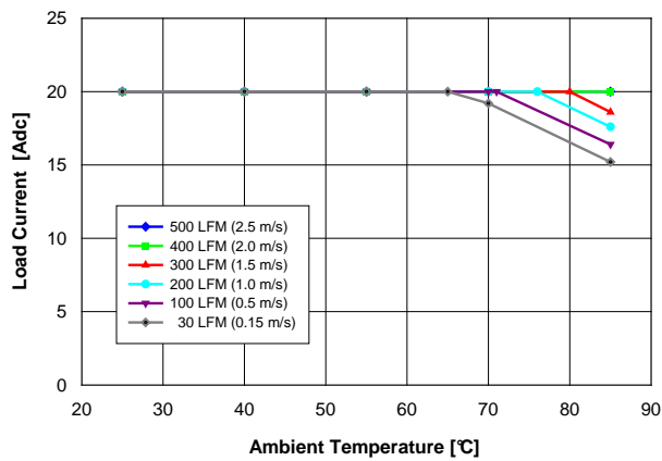
Figure 1. Available load current vs. ambient air temperature and airflow rates for SQL48T20033 converter mounted vertically with air flowing from pin 3 to pin 1, T_c temperatures \leq 120 °C, V_{in} = 48 V.
