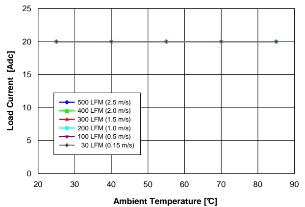
Figure 3. Power derating of SQL48T20033 converter with baseplate option and 0.91" tall horizontal-fin heatsink. (Conditions: same as Figure 1) No thermal derating required.
