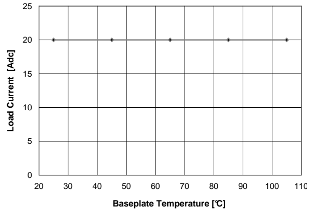
Figure 4. Coldplate cooling: Power derating of SQL48T20033-xxx Bx converter with baseplate option and coldplate cooling. (Conditions: Air velocity \leq 30 LFM ( \leq 0.15 m/s), V_{in} = 48 V, T_B \leq 105 °C)
