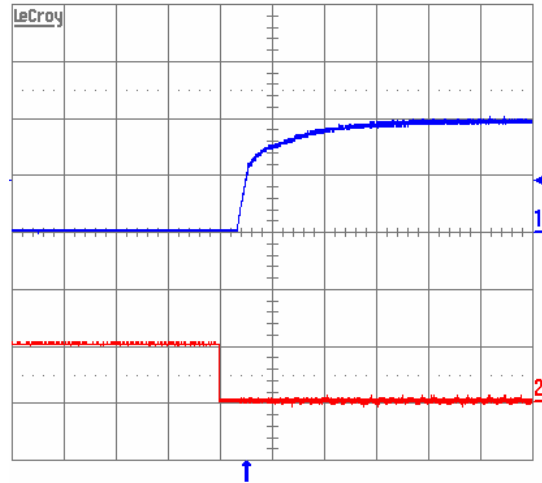
Figure 7. Turn-on transient at full rated load current (resistive) plus 10,000 µF at Vin = 48 V, 30 Amps and turned on using ON/OFF pin. Top trace, Iout=Output voltage (0.5 V/div.). Bottom trace: ON/OFF signal (5 V/div.). Time scale: 2 ms/div.
