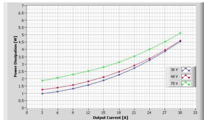
Figure 3. Power dissipation vs. load current and for SQE48T30010 converter mounted horizontally. Convection cooled with T_a = 25^{\circ}\text{C} .
