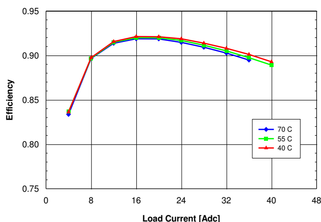
Figure 3. Efficiency vs. load current and ambient temperature for SQE48T40025 converter mounted vertically with V_{in}=48\text{V} and air flowing from pin 3 to pin 1 at 200LFM (1.0m/s).
