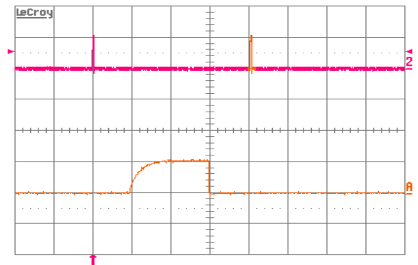
Figure 15. Load current (top trace, 50 A/div., 50 ms/div.) into a 10 \text{ m}\Omega short circuit during restart, at V_{in} = 48 \text{ V} . Bottom trace (50 A/div., 1 ms/div.) is an expansion of the on-time portion of the top trace.
