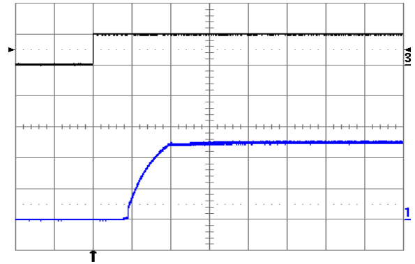
Fig. 2.5V.4: Turn-on transient at full rated load current (resistive) plus 10,000 \mu F at V_{in} = 48 V, triggered via ON/OFF pin. Top trace: ON/OFF signal (5 V/div.). Bottom trace: output voltage (1 V/div.). Time scale: 2 ms/div.
