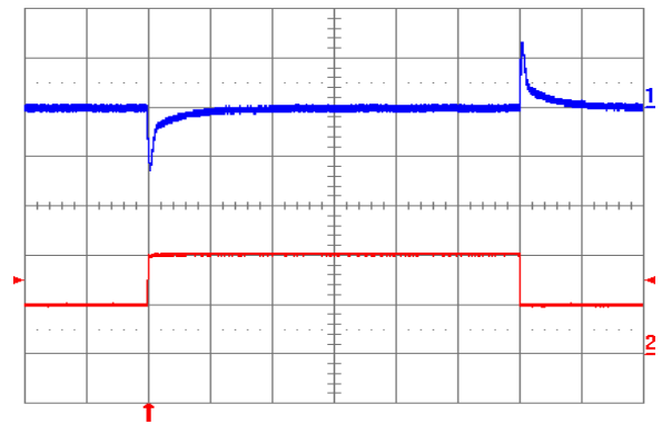
Fig. 2.5V.6: Output voltage response to load current step-change (5A – 10A – 5A) at V_{in} = 48 V. Top trace: output voltage (100 mV/div.). Bottom trace: load current (5 A/div.). Current slew rate: 5 A/ \mu s. C_o = 450 \mu F tantalum + 1 \mu F ceramic. Time scale: 0.2 ms/div.
