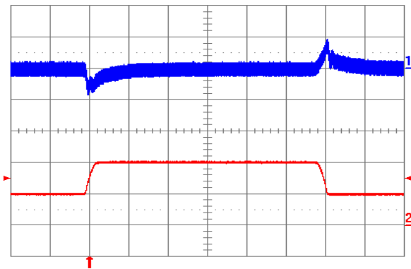
Fig. 2.5V.5: Output voltage response to load current step-change (5A – 10A – 5A) at V_{in} = 48 V. Top trace: output voltage (100 mV/div.). Bottom trace: load current (5 A/div.). Current slew rate: 0.1 A/ \mu s. C_o = 1 \mu F ceramic. Time scale: 0.2 ms/div.
