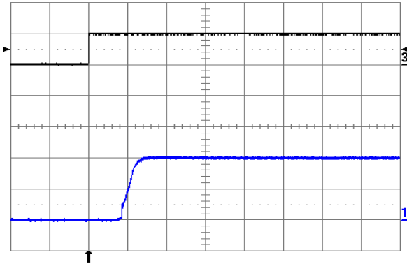
Fig. 2.0V.3: Turn-on transient at full rated load current (resistive) with no output capacitor at V_{in} = 48 V, triggered via ON/OFF pin. Top trace: ON/OFF signal (5 V/div.). Bottom trace: output voltage (1 V/div.). Time scale: 2 ms/div.
