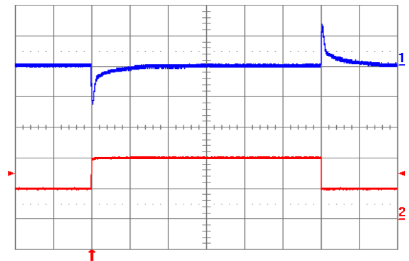
Fig. 2.0V.6: Output voltage response to load current step-change (5A – 10A – 5A) at V_{in} = 48 V. Top trace: output voltage (100 mV/div.). Bottom trace: load current (5 A/div.). Current slew rate: 5 A/ \mu s. C_o = 450 \mu F tantalum + 1 \mu F ceramic. Time scale: 0.2 ms/div.
