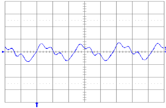
Fig. 3.3V.7: Output voltage ripple (20 mV/div.) at full rated load current into a resistive load with C_o = 10 \mu\text{F} tantalum + 1 \mu\text{F} ceramic and V_{in} = 48 \text{ V} . Time scale: 1 \mu\text{s}/\text{div} .
