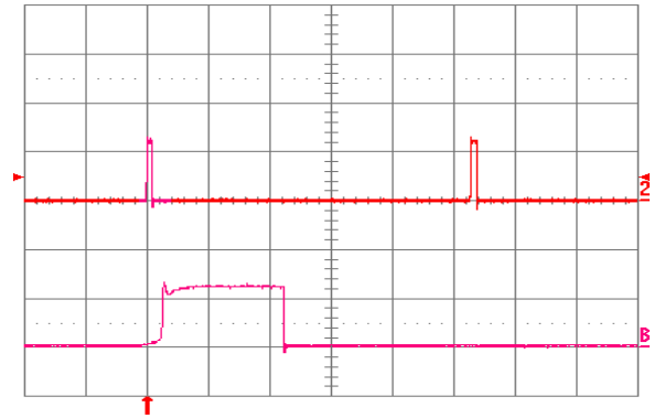
Fig. 2.0V.12: Load current (top trace, 20 A/div., 20 ms/div.) into a 10 m \Omega short circuit during restart, at V_{in} = 48 V. Bottom trace (20 A/div., 1 ms/div.) is an expansion of the on-time portion of the top trace.
