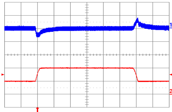
Fig. 2.0V.5: Output voltage response to load current step-change (5A – 10A – 5A) at V_{in} = 48 V. Top trace: output voltage (100 mV/div.). Bottom trace: load current (5A/div.). Current slew rate: 0.1 A/ \mu s. C_o = 1 \mu F ceramic. Time scale: 0.2 ms/div.
