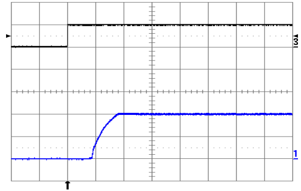
Fig. 2.0V.4: Turn-on transient at full rated load current (resistive) plus 10,000 \mu F at V_{in} = 48 V, triggered via ON/OFF pin. Top trace: ON/OFF signal (5 V/div.). Bottom trace: output voltage (1 V/div.). Time scale: 2 ms/div.
