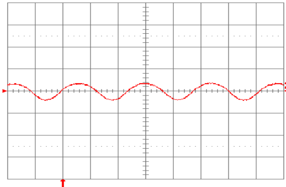
Fig. 1.8V.9: Input reflected ripple current, i_c (100 mA/div.), measured at input terminals at full rated load current and V_{in} = 48 \text{ V} . Refer to Fig. 1.8V.8 for test setup. Time scale: 1 \mu\text{s}/\text{div.}
