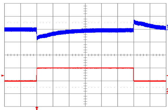
Fig. 6.0V.12: Output voltage response to load current step-change (2A – 4A – 2A) at V_{in} = 24V . Top trace: output voltage (100mV/div.). Bottom trace: load current (2A/div.). Current slew rate: 5 A/µs. C_o = 450 \mu F tantalum + 1 µF ceramic. Time scale: 0.2 ms/div.
