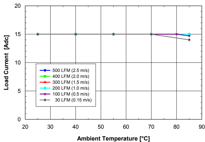
Fig. 2.0V.4: Available load current vs. ambient temperature and airflow rates for ASQ24S15020 converter mounted horizontally with V_{in} = 24V , air flowing from pin 3 to pin 1 and maximum FET temperature \leq 120^{\circ}C .
