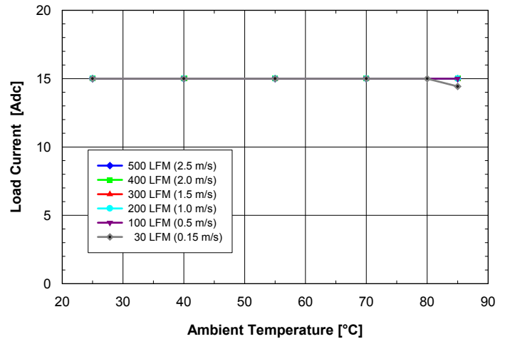
Fig. 1.8V.2: Available load current vs. ambient air temperature and airflow rates for ASQ24T15018 converter with B height pins mounted horizontally with V_{in} = 24V , air flowing from pin 3 to pin 1 and maximum FET temperature \leq 120^{\circ}C .
