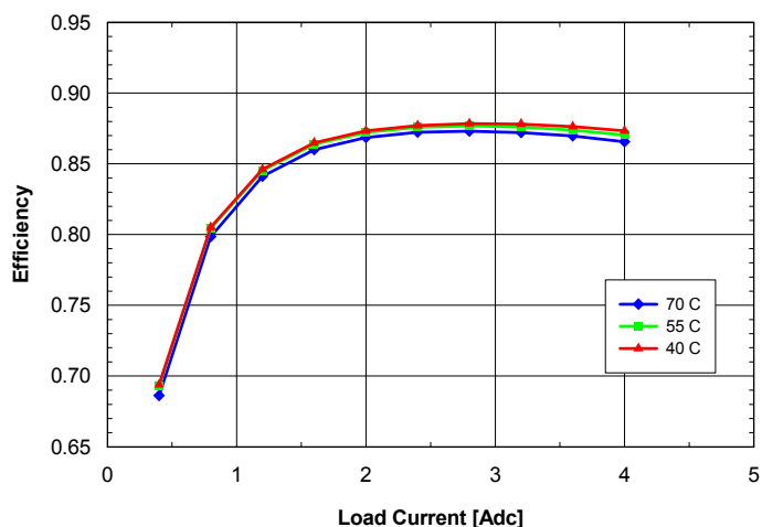
Fig. 12V.6: Efficiency vs. load current and ambient temperature for ASQ24T/S04120 converter mounted vertically with V_{in} = 24\text{V} and air flowing from pin 3 to pin 1 at a rate of 200 LFM (1.0 m/s).
