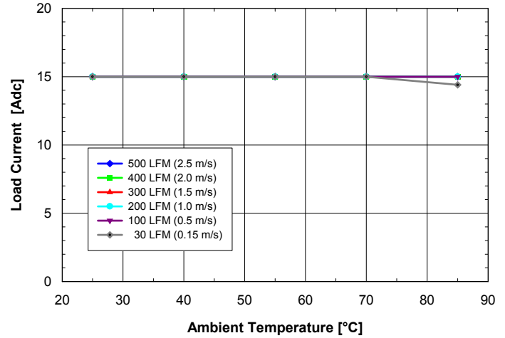
Fig. 1.8V.4: Available load current vs. ambient temperature and airflow rates for ASQ24S15018 converter mounted horizontally with V_{in} = 24V , air flowing from pin 3 to pin 1 and maximum FET temperature \leq 120^{\circ}C .
