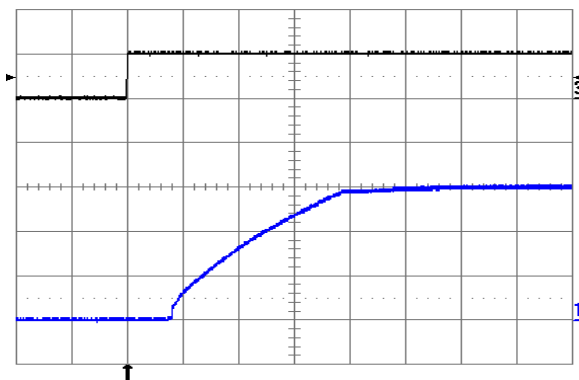
Fig. 6.0V.10: Turn-on transient at full rated load current (resistive) plus 10,000µF at V_{in} = 24V , triggered via ON/OFF pin. Top trace: ON/OFF signal (5 V/div.). Bottom trace: output voltage (2 V/div.). Time scale: 2 ms/div.
