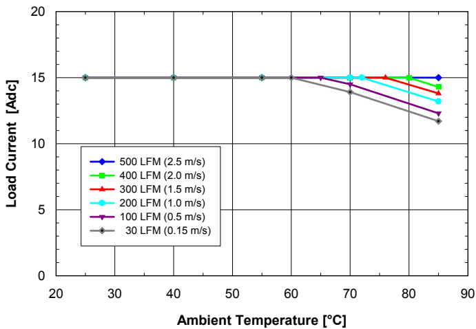
Fig. 11: Available load current vs. ambient temperature and airflow rates for ASQ48S15018 converter mounted vertically with V_{in} = 48\text{ V} , air flowing from pin 3 to pin 1 and maximum FET temperature \leq 120^{\circ}\text{C} .
