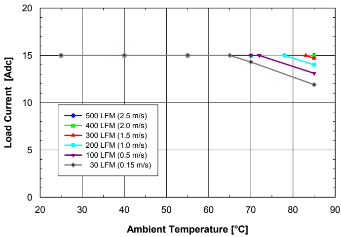
Fig. 9: Available load current vs. ambient air temperature and airflow rates for ASQ48T15018 converter with D height pins mounted vertically with V_{in} = 48\text{ V} , air flowing from pin 3 to pin 1 and maximum FET temperature \leq 120^{\circ}\text{C} .
