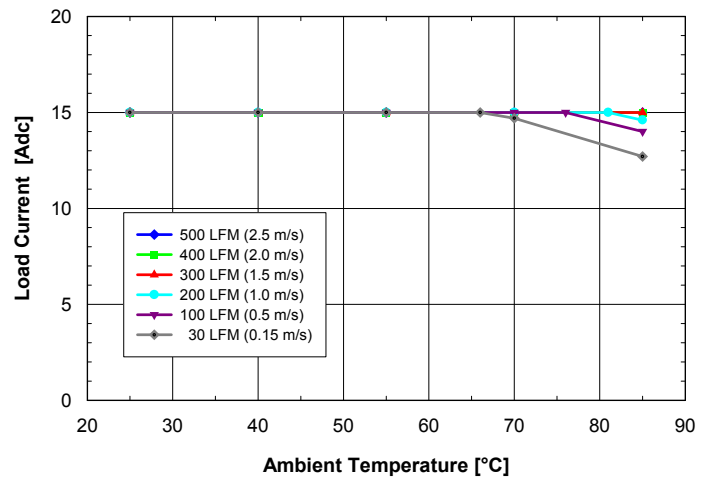
Fig. 10: Available load current vs. ambient air temperature and airflow rates for ASQ48T15018 converter with D height pins mounted horizontally with V_{in} = 48\text{ V} , air flowing from pin 3 to pin 1 and maximum FET temperature \leq 120^{\circ}\text{C} .
