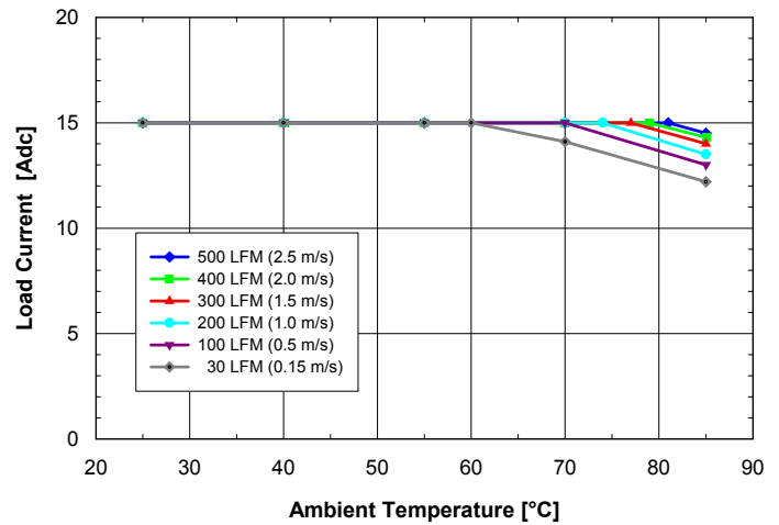
Fig. 12: Available load current vs. ambient temperature and airflow rates for ASQ48S15018 converter mounted horizontally with V_{in} = 48\text{ V} , air flowing from pin 3 to pin 1 and maximum FET temperature \leq 120^{\circ}\text{C} .
