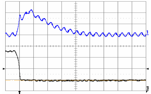
Fig. 10b*: Output voltage response to load current step-change (10 A – 15 A – 10 A) at V_{in} = 48 V. Top trace: output voltage (50 mV/div.). Bottom trace: load current (2 A/div.). Current slew rate: 2.5 A/ \mu s. C_o = 2 \times 100 \mu F TA + 1 \mu F ceramic. Time scale: 5 \mu s/div.
