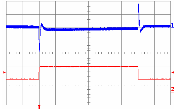
Fig. 10: Output voltage response to load current step-change (10 A – 20 A – 10 A) at V_{in} = 48 V. Top trace: output voltage (100 mV/div.). Bottom trace: load current (10 A/div.). Current slew rate: 5 A/ \mu s. C_o = 470 \mu F POS + 1 \mu F ceramic. Time scale: 0.2 ms/div.
