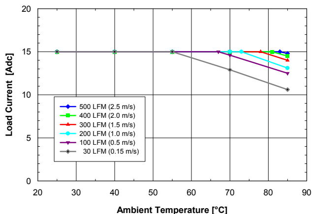
Fig. 2.5V.2: Available load current vs. ambient air temperature and airflow rates for SQ48T15025 converter with D height pins mounted horizontally with V_{in} = 48\text{ V} , air flowing from pin 3 to pin 1, and maximum FET temperature \leq 120^\circ\text{C} .
