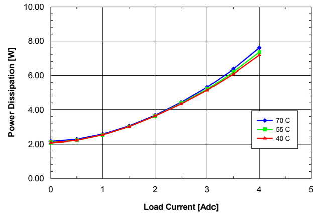
Fig. 12V.8: Power dissipation vs. load current and ambient temperature for SQ48T/S04120 converter mounted vertically with V_{in} = 48\text{ V} and air flowing from pin 3 to pin 1 at a rate of 200 LFM (1.0 m/s).
