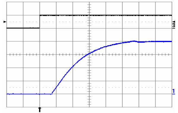
Fig. 8.0V.10: Turn-on transient at full rated load current (resistive) plus 2,200 \mu\text{F} at V_{in} = 48\text{ V} , triggered via ON/OFF pin. Top trace: ON/OFF signal (5 V/div.). Bottom trace: output voltage (2 V/div.). Time scale: 2 ms/div.
