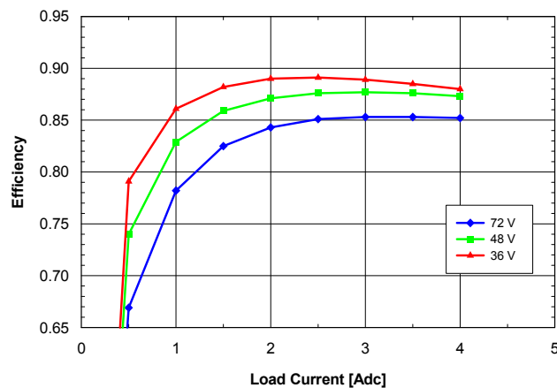
Fig. 12V.5: Efficiency vs. load current and input voltage for SQ48T/S04120 converter mounted vertically with air flowing from pin 3 to pin 1 at a rate of 300 LFM (1.5 m/s) and T_a = 25 °C.
