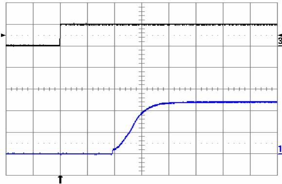
Fig. 12V.9: Turn-on transient at full rated load current (resistive) with no output capacitor at V_{in} = 48\text{ V} , triggered via ON/OFF pin. Top trace: ON/OFF signal (5 V/div.). Bottom trace: output voltage (5 V/div.). Time scale: 1 ms/div.
