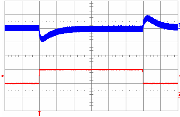
Fig. 12V.11: Output voltage response to load current step-change (1 A – 2 A – 1 A) at V_{in} = 48 V. Top trace: output voltage (200 mV/div.). Bottom trace: load current (1 A/div.). Current slew rate: 0.1 A/ \mu s. C_o = 1 \mu F ceramic. Time scale: 0.5 ms/div.
