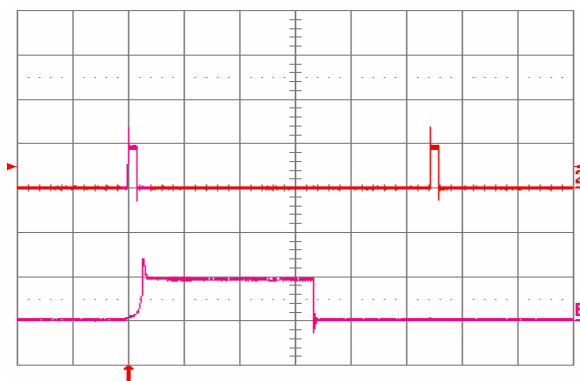
Fig. 1.0V.18: Load current (top trace, 20 A/div., 20 ms/div.) into a 10 m \Omega short circuit during restart, at V_{in} = 48 V. Bottom trace (20 A/div., 1 ms/div.) is an expansion of the on-time portion of the top trace.
