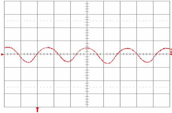
Fig. 8.0V.15: Input reflected ripple current, i_c (100 mA/div.), measured at input terminals at full rated load current and V_{in} = 48 V. Refer to Fig. 8.0V.14 for test setup. Time scale: 1 \mu s/div.
