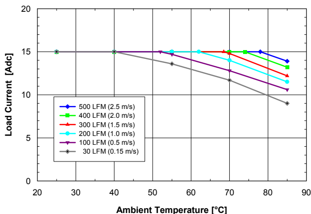
Fig. 3.3V.1: Available load current vs. ambient air temperature and airflow rates for SQ48T15033 converter with D height pins mounted vertically with V_{in} = 48\text{ V} , air flowing from pin 3 to pin 1, and maximum FET temperature \leq 120^\circ\text{C} .
