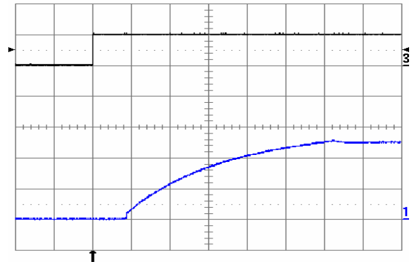
Fig. 5.0V.10: Turn-on transient at full rated load current (resistive) plus 10,000 \mu\text{F} at V_{in} = 48\text{ V} , triggered via ON/OFF pin. Top trace: ON/OFF signal (5 V/div.). Bottom trace: output voltage (2 V/div.). Time scale: 2 ms/div.
