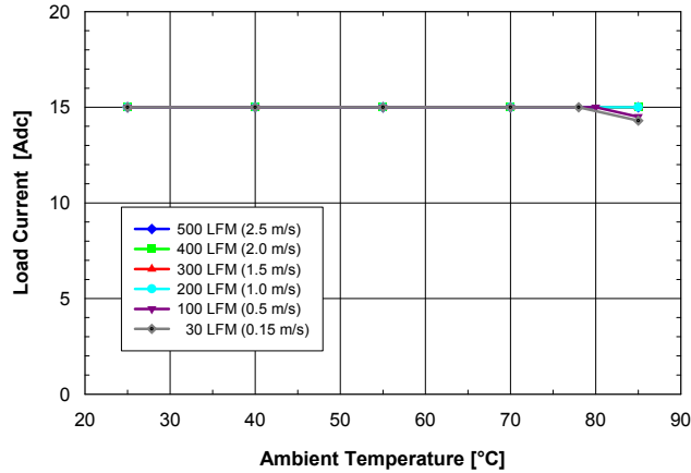
Fig. 1.2V.3: Available load current vs. ambient air temperature and airflow rates for SQ48S15012 converter mounted vertically with V_{in} = 48 V, air flowing from pin 3 to pin 1, and maximum FET temperature \leq 120 °C.
