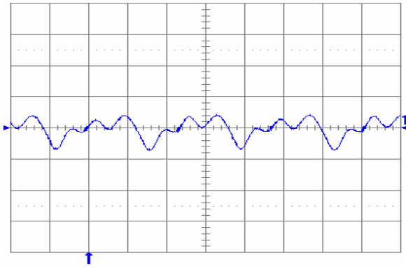
Fig. 2.0V.13: Output voltage ripple (20 mV/div.) at full rated load current into a resistive load with C_o = 10 μF tantalum + 1 μF ceramic and V_{in} = 48 V. Time scale: 1 μs/div.
