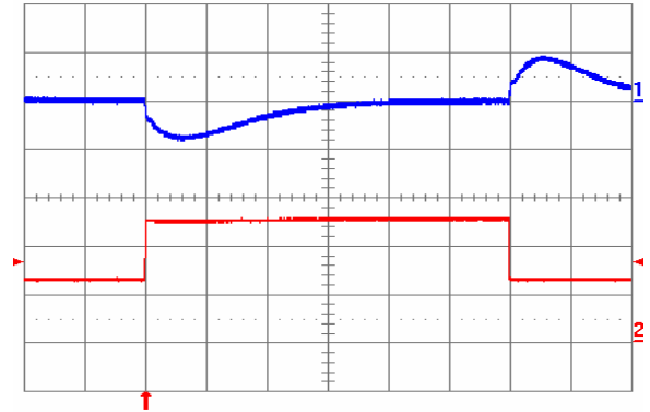
Fig. 5.0V.12: Output voltage response to load current step-change (2.5 A – 5 A – 2.5 A) at V_{in} = 48 V. Top trace: output voltage (200 mV/div.). Bottom trace: load current (2 A/div.). Current slew rate: 5 A/ \mu s. C_o = 450 \mu F tantalum + 1 \mu F ceramic. Time scale: 0.2 ms/div.
