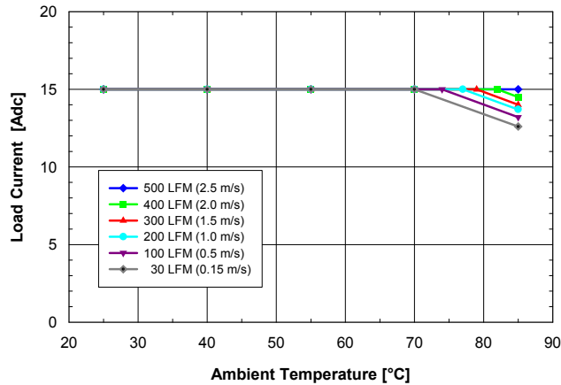
Fig. 2.0V.3: Available load current vs. ambient air temperature and airflow rates for SQ48S15020 converter mounted vertically with V_{in} = 48 V, air flowing from pin 3 to pin 1, and maximum FET temperature \leq 120 °C.
