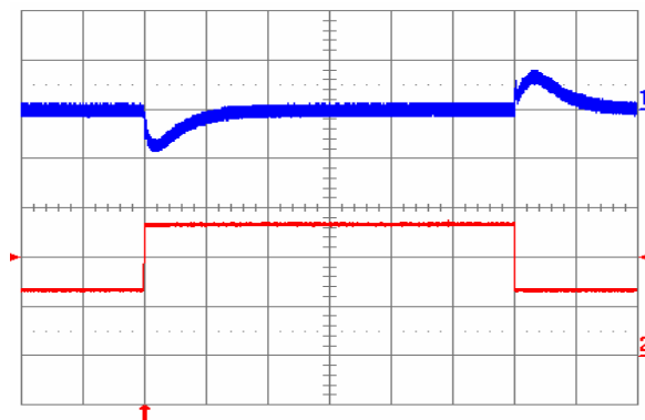
Fig. 8.0V.12: Output voltage response to load current step-change (1.325 A – 2.65 A – 1.325 A) at V_{in} = 48 V. Top trace: output voltage (200 mV/div.). Bottom trace: load current (1 A/div.). Current slew rate: 5 A/ \mu s. C_o = 94 \mu F tantalum + 1 \mu F ceramic. Time scale: 0.5 ms/div.
