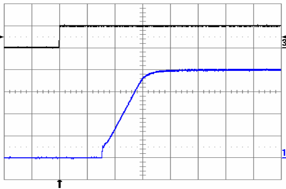
Fig. 8.0V.9: Turn-on transient at full rated load current (resistive) with no output capacitor at V_{in} = 48\text{ V} , triggered via ON/OFF pin. Top trace: ON/OFF signal (5 V/div.). Bottom trace: output voltage (2 V/div.). Time scale: 1 ms/div.
