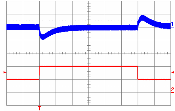
Fig. 12V.12: Output voltage response to load current step-change (1 A – 2 A – 1 A) at V_{in} = 48 V. Top trace: output voltage (200 mV/div.). Bottom trace: load current (1 A/div.). Current slew rate: 5 A/ \mu s. C_o = 47 \mu F tantalum + 1 \mu F ceramic. Time scale: 0.5 ms/div.
