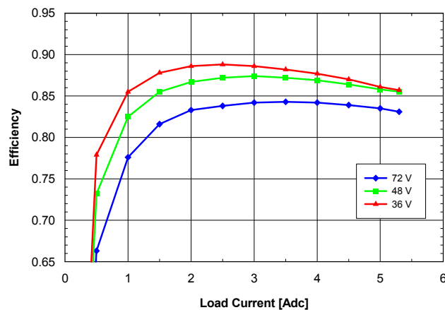
Fig. 8.0V.5: Efficiency vs. load current and input voltage for SQ48T/S05080 converter mounted vertically with air flowing from pin 3 to pin 1 at a rate of 300 LFM (1.5 m/s) and T_a = 25\text{ }^{\circ}\text{C} .
