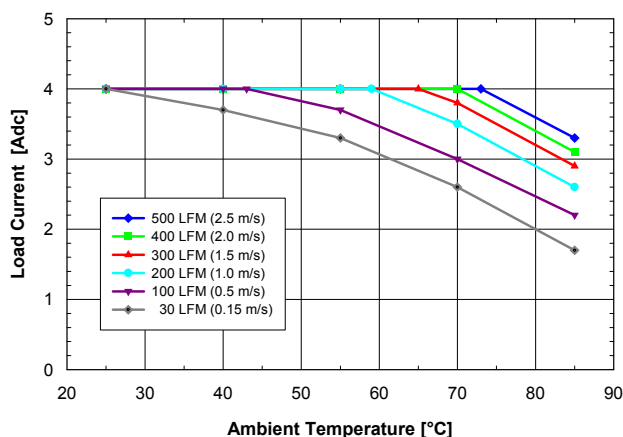
Fig. 12V.1: Available load current vs. ambient air temperature and airflow rates for SQ48T04120 converter with D height pins mounted vertically with V_{in} = 48\text{ V} , air flowing from pin 3 to pin 1, and maximum FET temperature \leq 120^\circ\text{C} .
