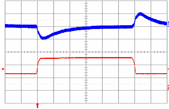
Fig. 5.0V.11: Output voltage response to load current step-change (2.5 A – 5 A – 2.5 A) at V_{in} = 48 V. Top trace: output voltage (200 mV/div.). Bottom trace: load current (2 A/div.). Current slew rate: 0.1 A/ \mu s. C_o = 1 \mu F ceramic. Time scale: 0.2 ms/div.
