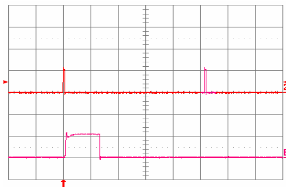
Fig. 6.0V.18: Load current (top trace, 10 A/div., 20 ms/div.) into a 10 m\Omega short circuit during restart, at V_{in} = 48 V. Bottom trace (10 A/div., 1 ms/div.) is an expansion of the on-time portion of the top trace.
