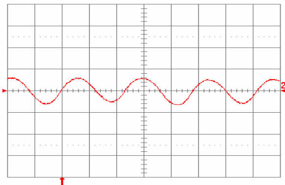
Fig. 5.0V.15: Input reflected ripple current, i_c (100 mA/div.), measured at input terminals at full rated load current and V_{in} = 48 V. Refer to Fig. 5.0V.14 for test setup. Time scale: 1 \mu s/div.
