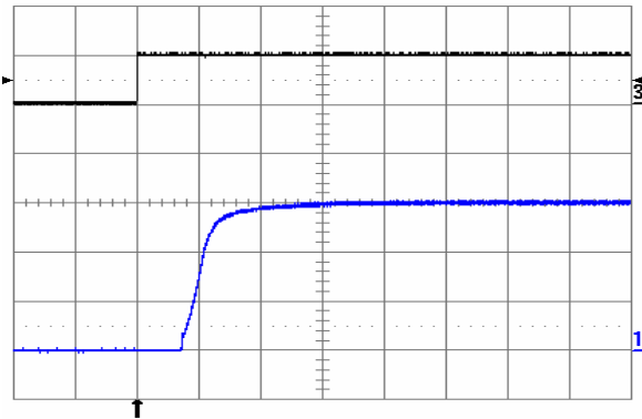
Fig. 6.0V.9: Turn-on transient at full rated load current (resistive) with no output capacitor at V_{in} = 48\text{ V} , triggered via ON/OFF pin. Top trace: ON/OFF signal (5 V/div.). Bottom trace: output voltage (2 V/div.). Time scale: 2 ms/div.
