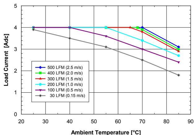
Fig. 12V.2: Available load current vs. ambient air temperature and airflow rates for SQ48T04120 converter with D height pins mounted horizontally with V_{in} = 48\text{ V} , air flowing from pin 3 to pin 1, and maximum FET temperature \leq 120^\circ\text{C} .
