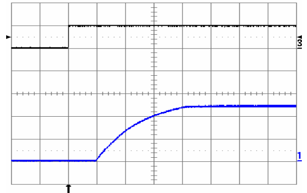
Fig. 12V.10: Turn-on transient at full rated load current (resistive) plus 1,000 \mu\text{F} at V_{in} = 48\text{ V} , triggered via ON/OFF pin. Top trace: ON/OFF signal (5 V/div.). Bottom trace: output voltage (5 V/div.). Time scale: 2 ms/div.
