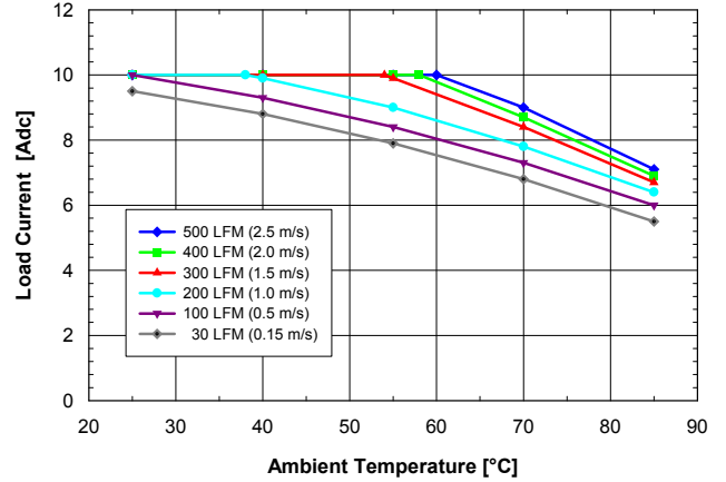
Fig. 5.0V.4: Available load current vs. ambient air temperature and airflow rates for SQ48S10050 converter mounted horizontally with V_{in} = 48\text{ V} , air flowing from pin 3 to pin 1, and maximum FET temperature \leq 120\text{ }^{\circ}\text{C} .
