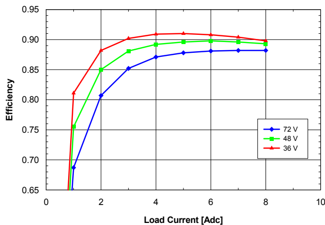
Fig. 6.0V.5: Efficiency vs. load current and input voltage for SQ48T/S08060 converter mounted vertically with air flowing from pin 3 to pin 1 at a rate of 300 LFM (1.5 m/s) and T_a = 25 °C.
