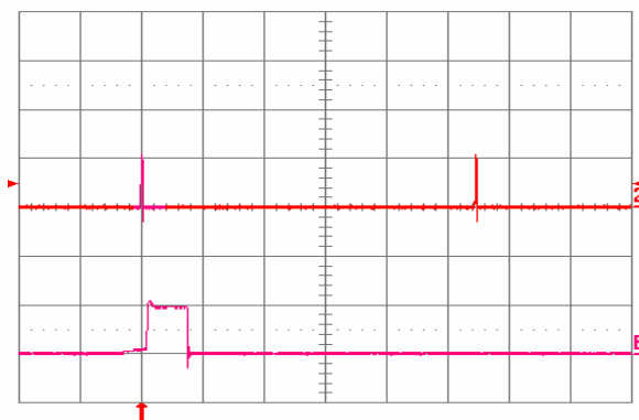
Fig. 2.0V.18: Load current (top trace, 20 A/div., 20 ms/div.) into a 10 m \Omega short circuit during restart, at V_{in} = 48 V. Bottom trace (20 A/div., 1 ms/div.) is an expansion of the on-time portion of the top trace.
