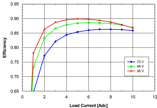
Fig. 5.0V.5: Efficiency vs. load current and input voltage for SQ48T/S10050 converter mounted vertically with air flowing from pin 3 to pin 1 at a rate of 300 LFM (1.5 m/s) and T_a = 25\text{ }^{\circ}\text{C} .
