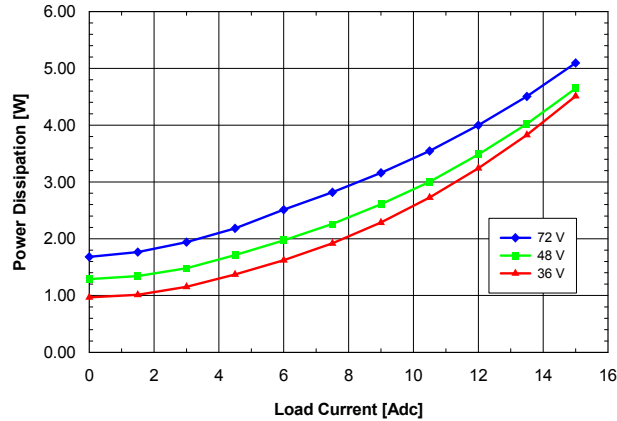
Fig. 2.0V.7: Power dissipation vs. load current and input voltage for SQ48T/S15020 converter mounted vertically with air flowing from pin 3 to pin 1 at a rate of 300 LFM (1.5 m/s) and T_a = 25^\circ\text{C} .
