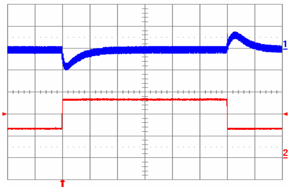
Fig. 8.0V.11: Output voltage response to load current step-change (1.325 A – 2.65 A – 1.325 A) at V_{in} = 48 V. Top trace: output voltage (200 mV/div.). Bottom trace: load current (1 A/div.). Current slew rate: 0.1 A/ \mu s. C_o = 1 \mu F ceramic. Time scale: 0.5 ms/div.
