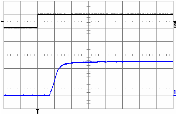
Fig. 5.0V.9: Turn-on transient at full rated load current (resistive) with no output capacitor at V_{in} = 48\text{ V} , triggered via ON/OFF pin. Top trace: ON/OFF signal (5 V/div.). Bottom trace: output voltage (2 V/div.). Time scale: 2 ms/div.
