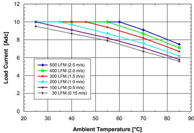
Fig. 5.0V.3: Available load current vs. ambient air temperature and airflow rates for SQ48S10050 converter mounted vertically with V_{in} = 48\text{ V} , air flowing from pin 3 to pin 1, and maximum FET temperature \leq 120\text{ }^{\circ}\text{C} .
