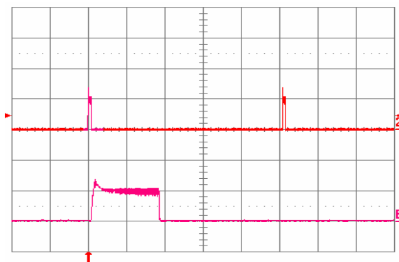
Fig. 12V.18: Load current (top trace, 5 A/div., 20 ms/div.) into a 10 m\Omega short circuit during restart, at V_{in} = 48 V. Bottom trace (5 A/div., 1 ms/div.) is an expansion of the on-time portion of the top trace.
