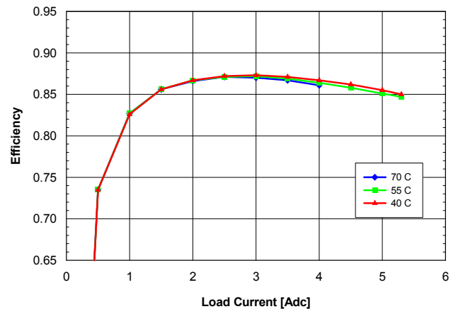
Fig. 8.0V.6: Efficiency vs. load current and ambient temperature for SQ48T/S05080 converter mounted vertically with V_{in} = 48\text{ V} and air flowing from pin 3 to pin 1 at a rate of 200 LFM (1.0 m/s).
