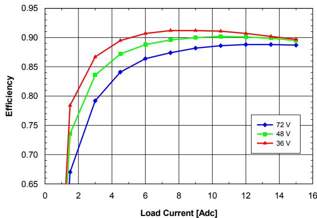
Fig. 3.3V.5: Efficiency vs. load current and input voltage for SQ48T/S15033 converter mounted vertically with air flowing from pin 3 to pin 1 at a rate of 300 LFM (1.5 m/s) and T_a = 25 °C.
