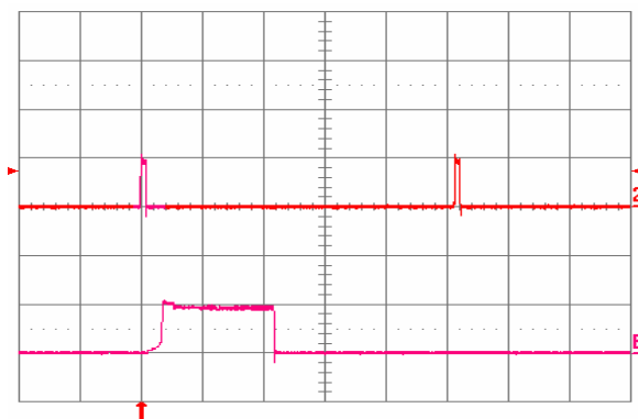
Fig. 3.3V.18: Load current (top trace, 20 A/div., 20 ms/div.) into a 10 m \Omega short circuit during restart, at V_{in} = 48 V. Bottom trace (20 A/div., 1 ms/div.) is an expansion of the on-time portion of the top trace.
