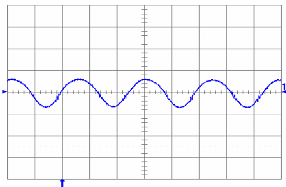
Fig. 8.0V.13: Output voltage ripple (50 mV/div.) at full rated load current into a resistive load with C_o = 10 \mu F tantalum + 1 \mu F ceramic and V_{in} = 48 V. Time scale: 1 \mu s/div.
