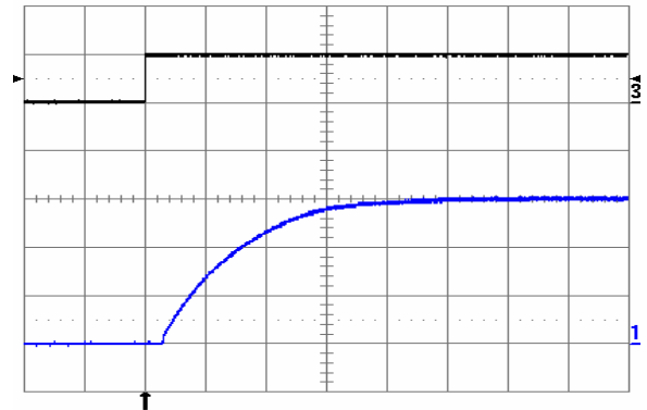
Fig. 6.0V.10: Turn-on transient at full rated load current (resistive) plus 10,000 \mu\text{F} at V_{in} = 48\text{ V} , triggered via ON/OFF pin. Top trace: ON/OFF signal (5 V/div.). Bottom trace: output voltage (2 V/div.). Time scale: 5 ms/div.
