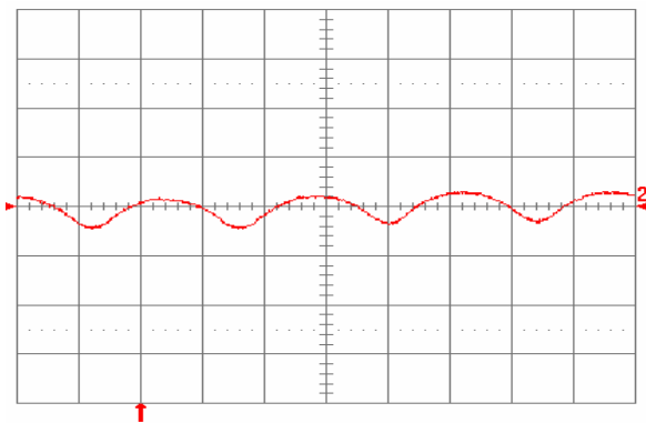
Fig. 1.0V.15: Input reflected ripple current, i_c (100 mA/div.), measured at input terminals at full rated load current and V_{in} = 48 V. Refer to Fig. 1.0V.14 for test setup. Time scale: 1 \mu s/div.
