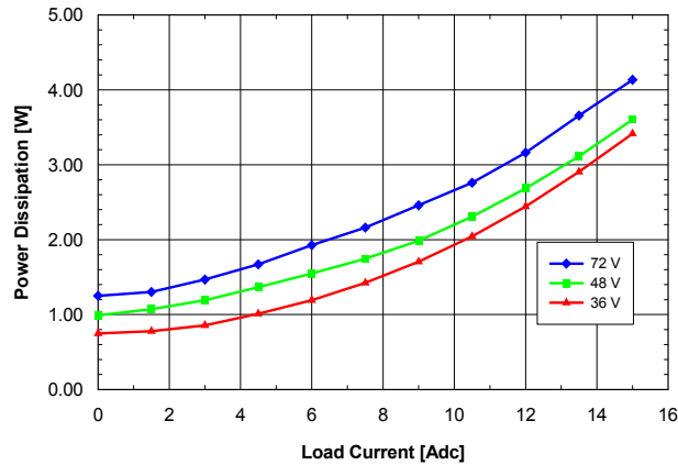
Fig. 1.0V.7: Power dissipation vs. load current and input voltage for SQ48T/S15010 converter mounted vertically with air flowing from pin 3 to pin 1 at a rate of 300 LFM (1.5 m/s) and T_a = 25^\circ\text{C} .
