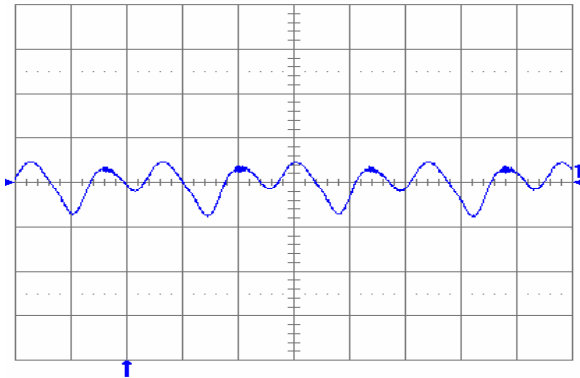
Fig. 1.5V.13: Output voltage ripple (20 mV/div.) at full rated load current into a resistive load with C_o = 10 μF tantalum + 1 μF ceramic and V_{in} = 48 V. Time scale: 1 μs/div.
