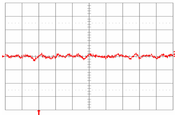
Fig. 1.0V.16: Input reflected ripple current, i_s (10 mA/div.), measured through 10 \mu H at the source at full rated load current and V_{in} = 48 V. Refer to Fig. 1.0V.14 for test setup. Time scale: 1 \mu s/div.
