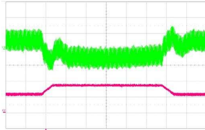
Fig. 11: Output voltage response to load current step change (23.5A – 35A – 23.5A) at V_{in} = 50\text{Vdc} . (Current Slew Rate: 0.1A/us. C_o = 10\mu\text{F} tantalum + 1uF ceramic). Top Trace: Output Voltage (100mV/div). Bottom Trace: Load Current (20A/div). Time Scale: 0.2 ms/div.
