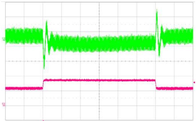
Fig. 12: Output voltage response to load current step change (23.5A – 35A – 23.5A) at V_{in} = 50\text{ Vdc} . (Current Slew Rate: 1A/us. C_o = 180\mu\text{F} ). Top Trace: Output Voltage (200mV/div). Bottom Trace: Load Current (20A/div). Time Scale: 0.2 ms/div.
