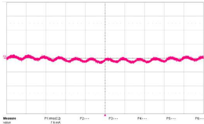
Fig. 15: Input reflected ripple current ( i_s ) measured through a 5 \mu\text{H} inductor / 470 \mu\text{F} capacitor filter at the source at full rated load current and V_{in} = 50 \text{ Vdc} . Vertical Axis: 50 \text{ mA}/\text{div} . Time Scale: 5 \mu\text{s}/\text{div} .
