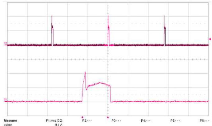
Fig. 16: Load Current into 10 \text{ m}\Omega load during short circuit test at V_{in} = 50 \text{ Vdc} . Top Trace: Load Current ( 50 \text{ A}/\text{div} , 100 \text{ ms}/\text{div} ). Bottom trace ( 50 \text{ A}/\text{div} , 5 \text{ ms}/\text{div} ) is an expansion of the on-time portion of the top trace.
