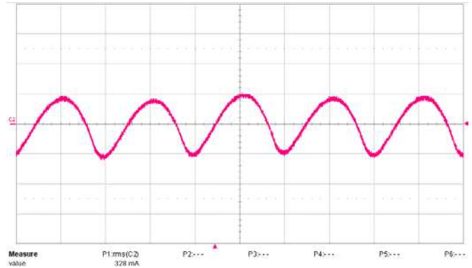
Fig. 14: Input ripple current ( i_{cin} ) measured at the input terminals at full rated load current and V_{in} = 50 \text{ Vdc} . Vertical Axis: 500 \text{ mA}/\text{div} . Time Scale: 2 \mu\text{s}/\text{div} .
