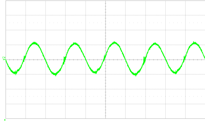
Fig. 13: Output voltage ripple (20 mV/div) at full rated load current into a resistive load with C_o = 750 \mu\text{F} , 25% ceramic, 75% OSCON or POSCAP and V_{in} = 50 \text{ Vdc} . Time Scale: 2 \mu\text{s}/\text{div} .
