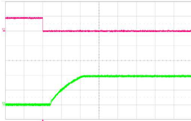
Fig. 9 Turn-on transient at full rated load current (resistive) with no output capacitor at V_{in} = 50\text{Vdc} , triggered via ON/OFF pin. Top Trace: ON/OFF Signal (5V/div). Bottom Trace: Output Voltage (5V/div). Time Scale: 5ms/div.
