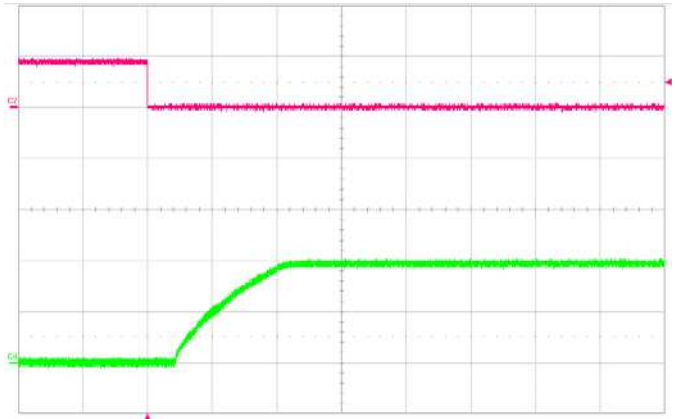
Fig. 10: Turn-on transient at full rated load current (resistive) plus 6,000uF output capacitor at V_{in} = 50\text{ Vdc} , triggered via ON/OFF pin. Top Trace: ON/OFF Signal (5V/div). Bottom Trace: Output Voltage (5V/div). Time Scale: 5ms/div.
