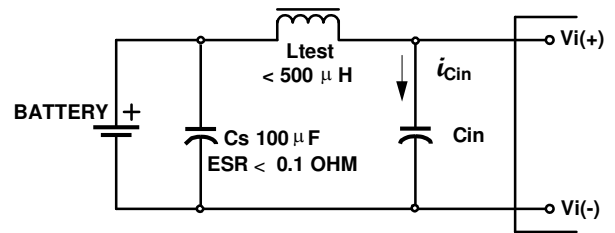
Figure C: Test set-up diagram showing the measurement of the input ripple current ( i_{cin} ) at the pins of the UUT.
