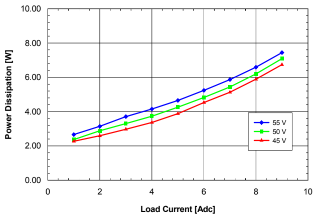
Fig. 9: Power dissipation vs. load current and input voltage for converter mounted vertically with air flowing from pin 3 to pin 1 at a rate of 200 LFM (1.5 m/s) and T_a = 25^\circ\text{C} .
