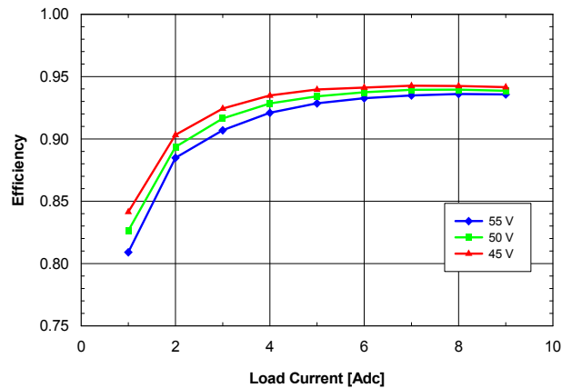
Fig. 7: Efficiency vs. load current and input voltage for converter mounted vertically with air flowing from pin 3 to pin 1 at a rate of 200 LFM (1.5 m/s) and T_a = 25^\circ\text{C} .
