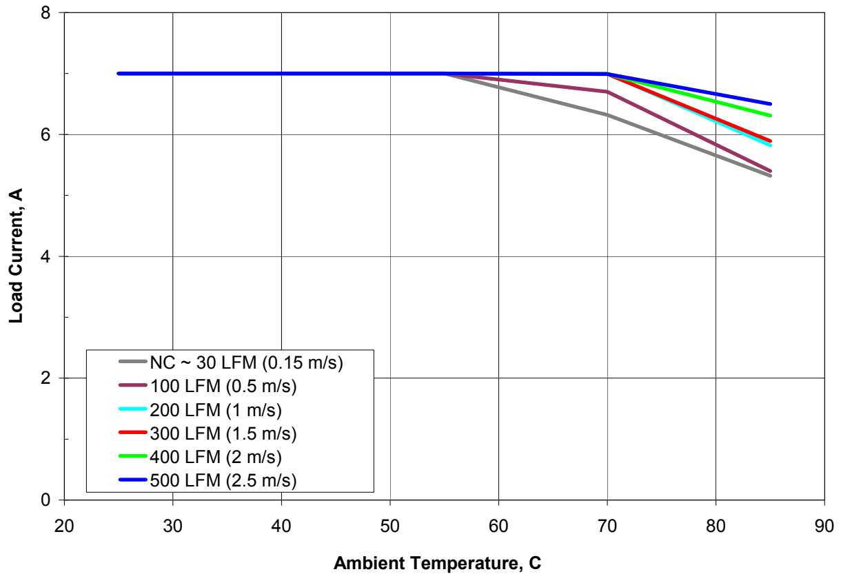
Figure 1. Available load current vs. ambient air temperature and airflow rates for SSQE48T07120 converter mounted vertically with air flowing from pin 1 to pin 3, V_{in} = 48\text{ V} . Note: NC – Natural convection
