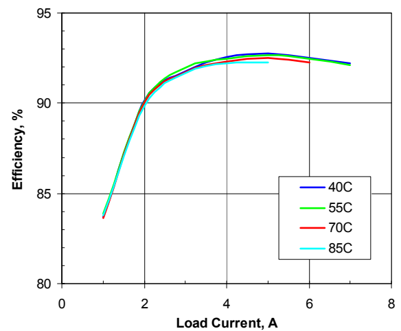
Figure 3. Efficiency vs. load current and ambient temperature for SSQE48T07120 converter mounted vertically with V_{in} = 48\text{ V} and air flowing from pin 1 to pin 3 at a rate of 200LFM (1.0m/s).
