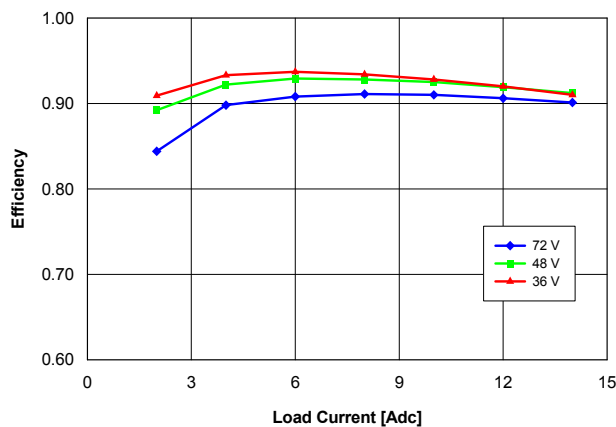
Fig. 3: Efficiency vs. load current and input voltage for converter mounted horizontally with air flowing from pin 3 to pin 1 at a rate of 300 LFM (1.5 m/s) and T_a = 25^{\circ}\text{C} .
