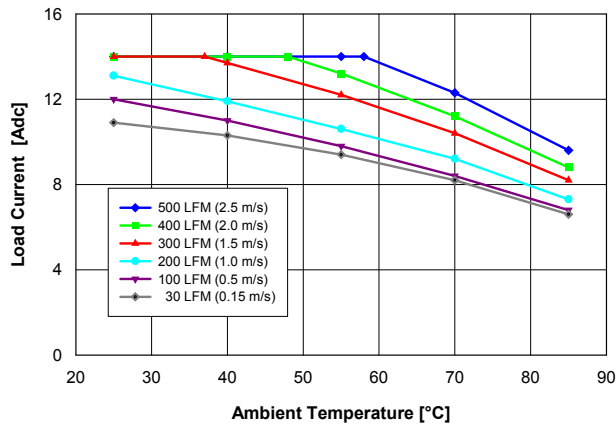
Fig. 1 : Available load current vs. ambient air temperature and airflow rates for converter with B height pins mounted vertically with air flowing from pin 3 to pin 1, MOSFET temperature \leq 120^{\circ}\text{C} , V_{in} = 48\text{ V} .
