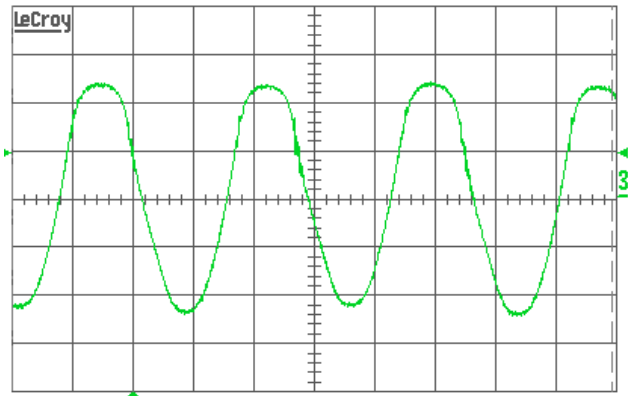
Fig. 13: Input reflected ripple current, i_c (200 mA/div.), measured at input terminals at full rated load current and V_{in} = 48 V. Refer to Fig. 12 for test setup. Time scale: 1 \mu s/div.
