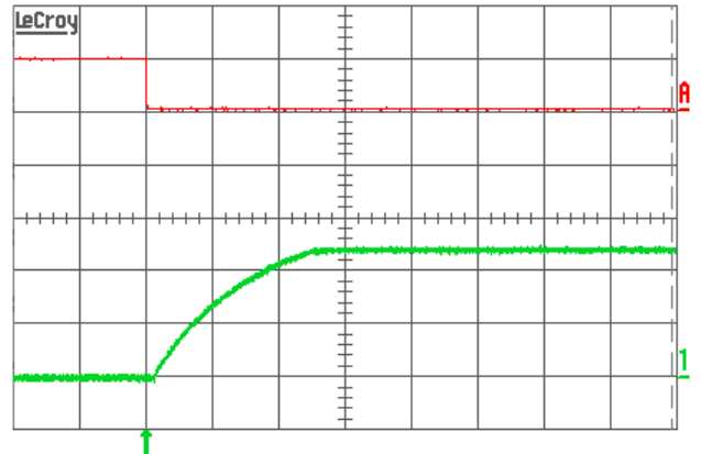
Fig. 8: Turn-on transient at full rated load current (resistive) plus 15,000 µF at V_{in} = 48\text{V} , triggered via ON/OFF pin. Top trace: ON/OFF signal (5 V/div.). Bottom trace: output voltage (5 V/div.). Time scale: 5 ms/div.
