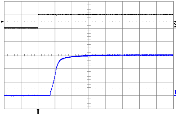
Fig. 6.0V.9: Turn-on transient at full rated load current (resistive) with no output capacitor at V_{in} = 48\text{V} , triggered via ON/OFF pin. Top trace: ON/OFF signal (5 V/div.). Bottom trace: output voltage (2V/div.). Time scale: 2 ms/div.
