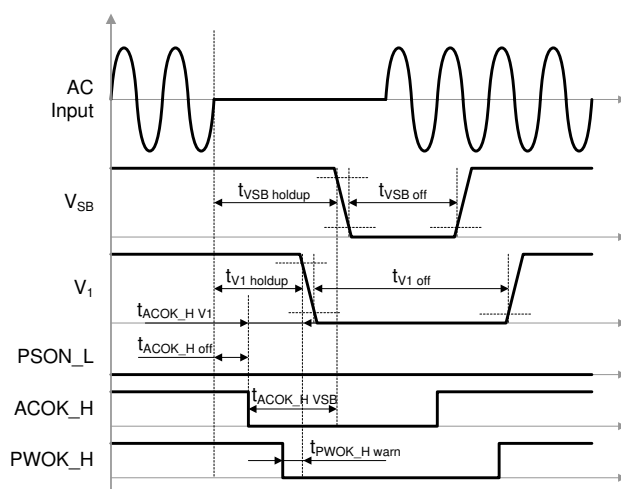
Figure 28: AC long dips
