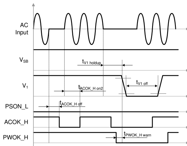
Figure 27: AC short dips
