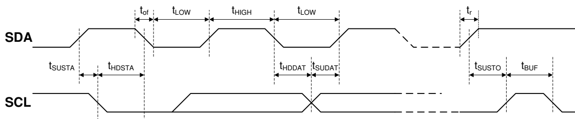
Figure 34: I 2 C / SMBus Timing
