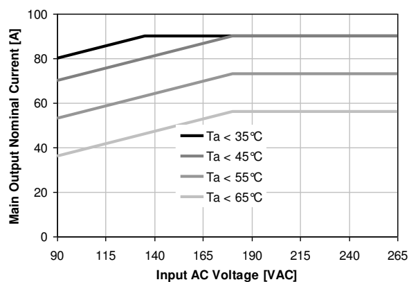
Figure 21: Derating on V_1 vs. V_i and T_a for PFE1100-12-054RA
