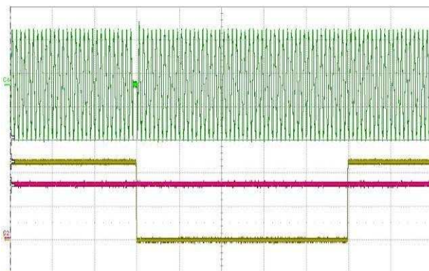
Figure 14: AC drop out 20 ms (200 ms/div), V_1 restart after 1 sec CH1: V_1 (5 V/div) CH2: V_{SB} (2 V/div) CH4: I_1 (200 V/div)
