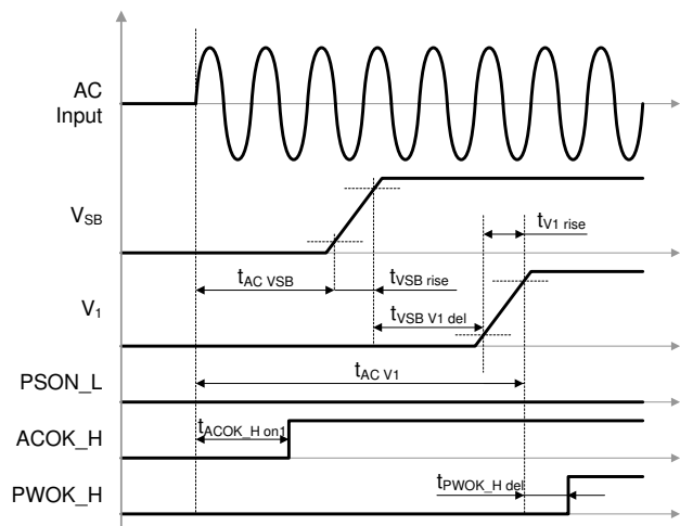
Figure 26: AC turn-on timing
