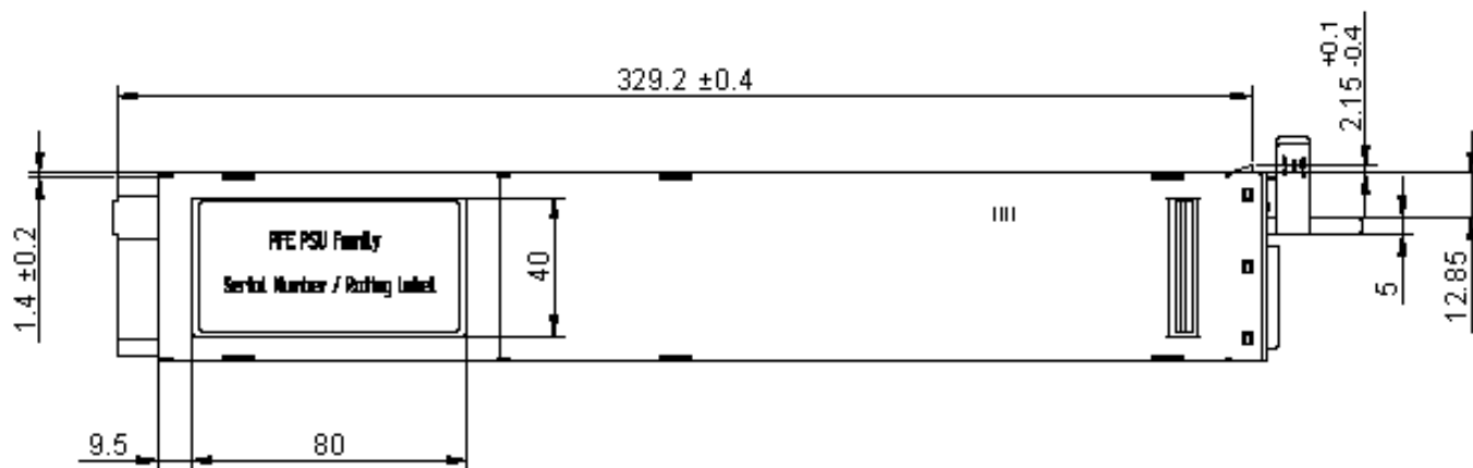
Figure 44: Top view
