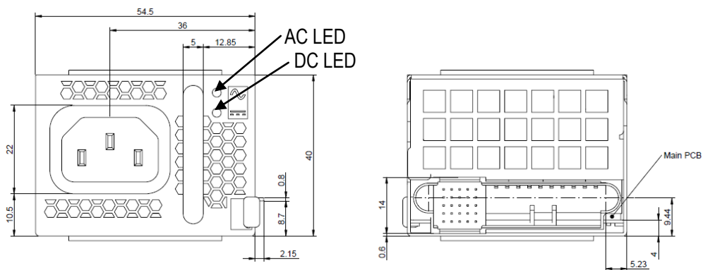
Figure 46: Front and rear view
