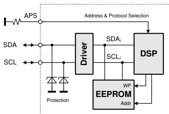
Figure 36: I²C Bus to DSP and EEPROM
