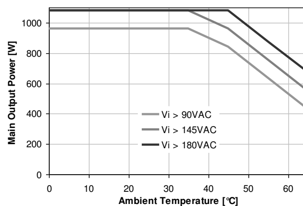
Figure 42: Thermal derating for PFE1100-12-054RA
