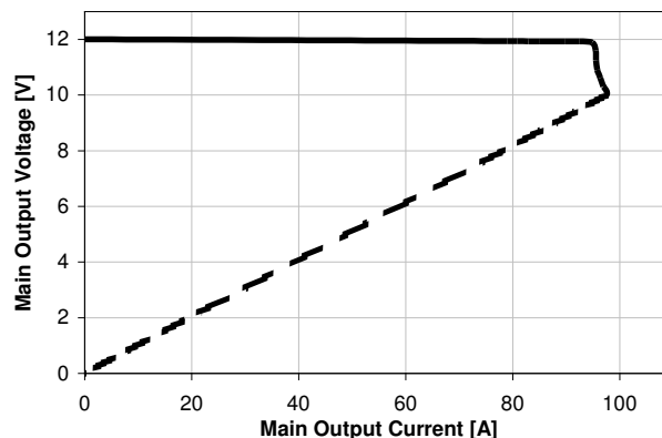
Figure 19: Current limitation on V_1 ( V_i = 230\text{ VAC} )
