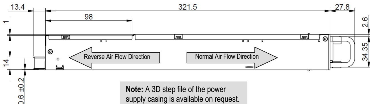
Figure 43: Side view 1
