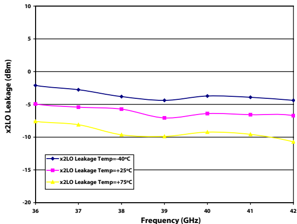
(x2)LO Leakage for XU1006-QB Vg2=-0.5V, Vd=4V, Id=240mA, P_LO=+4dBm, P_IF=-10dBm, IF_Frequency=2 GHz
