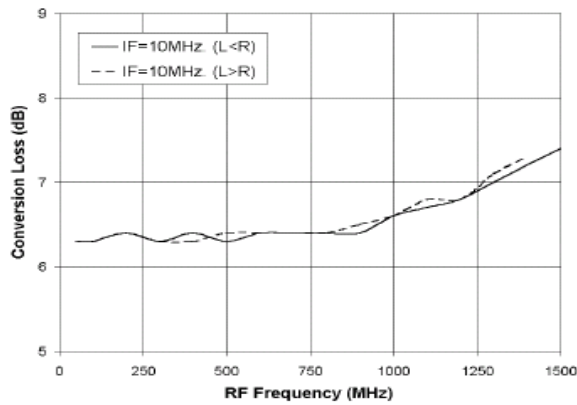
Conversion Loss vs. RF Frequency
