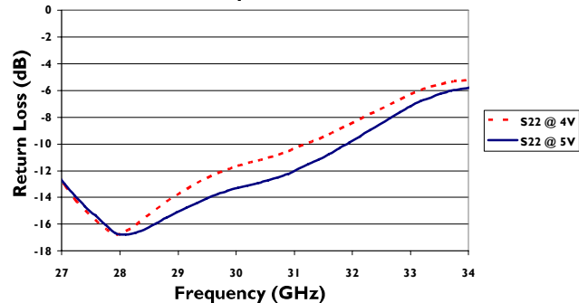
XX1007-QT: Input Return Loss (S22)
