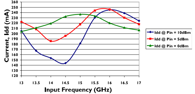
XX1007-QT: Idd Vs Input Frequency, Vd = 5V
