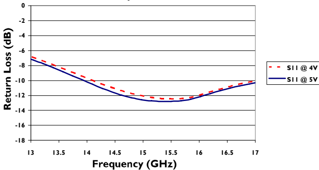
XX1007-QT: Input Return Loss (S11)
