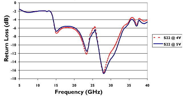
XX1007-QT: Input Return Loss (S22)
