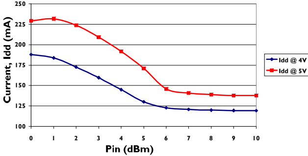
XX1007-QT: Idd Vs Pin, Input Frequency = 14.5 GHz
