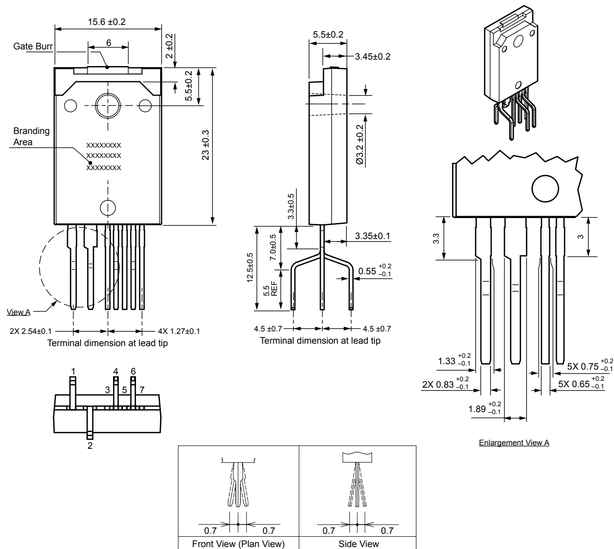
Package Outline Drawing, TO-3P
