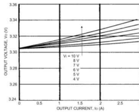
■ Load Regulation
