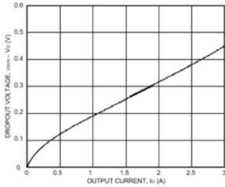
■ Dropout Voltage
