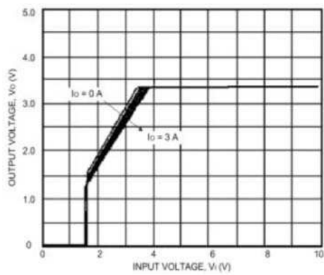
■ Low-Voltage Behavior
