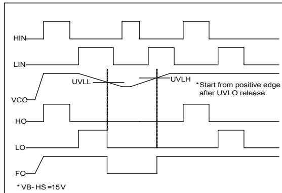
Low-Side Driver Input/Output
