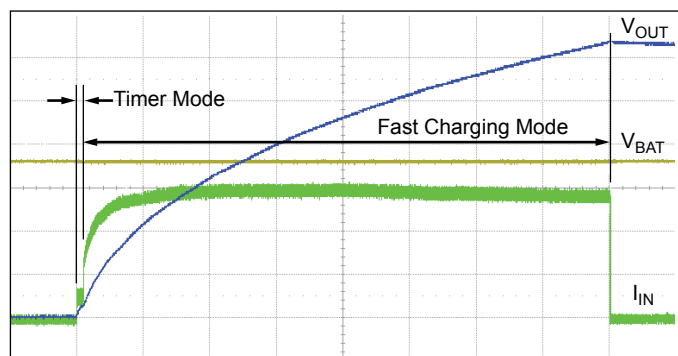
Figure 5. Timer Mode and Fast Charging Mode. t = 200\ \text{ms/div} , V_{OUT} = 50\ \text{V/div} , V_{BAT} = 1\ \text{V/div} , I_{IN} = 100\ \text{mA/div} , V_{BAT} = 3.6\ \text{V} , C_{OUT} = 20\ \mu\text{F}/330\ \text{V} , R_{SET} = 46\ \text{k}\Omega ( I_{SWlim} \approx 0.75\ \text{A} ).
