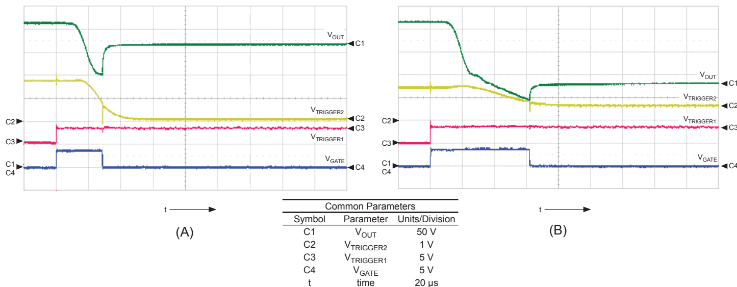
Figure 10. Adaptive timing of photoflash. (A) Subject near to camera, and (B) subject far from camera.
