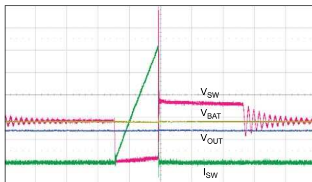
Figure 6. Timer Mode expanded view. V_{OUT} \leq 14\ \text{V} , t = 2\ \mu\text{s} / \text{div} , V_{BAT} = 3.6\ \text{V} , R_{SET} = 33.2\ \text{k}\Omega .
