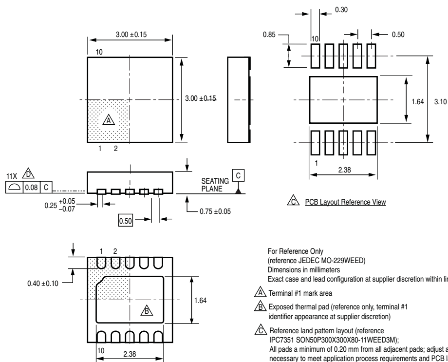
Package EJ, 3 mm x 3 mm 10-Contact DFN with Exposed Thermal Pad
