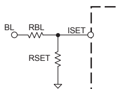
Figure 4. Smart Current Limit reference circuit
