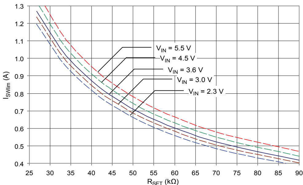
Figure 3. Peak Current Limit versus ISET Resistance. V_{IN} = V_{BAT} , transformer L_P = 8 \mu\text{H} , T_A = 25^\circ\text{C} .
