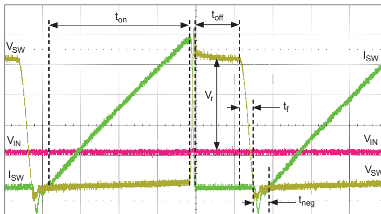
Figure 11. Pulse width relationship definitions.
