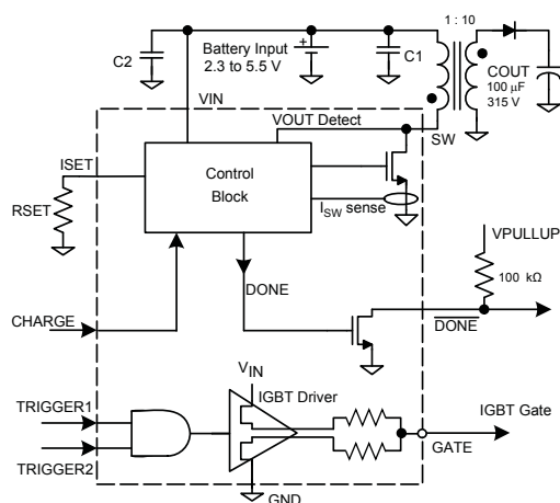
Figure 1. Typical application with separate trigger inputs.
