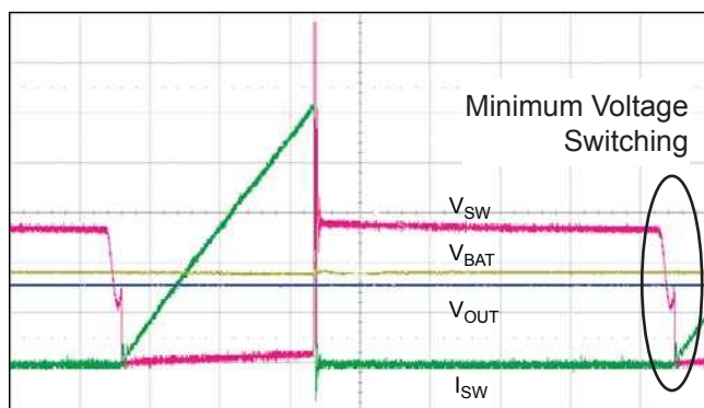
Figure 7. Minimum voltage switching. V_{OUT} \geq 15\ \text{V} ; t = 1\ \mu\text{s}/\text{div.} , V_{BAT} = 3.6\ \text{V} , R_{SET} = 33.2\ \text{k}\Omega .
