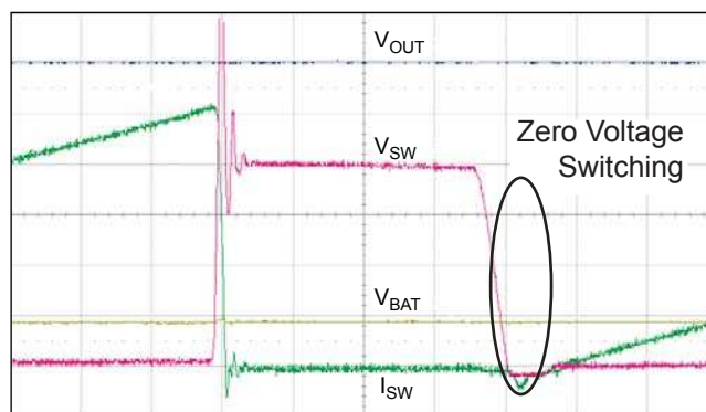
Figure 8. Zero voltage switching. V_{OUT} = 120\ \text{V} . t = 0.2\ \mu\text{s}/\text{div.} , V_{BAT} = 3.6\ \text{V} , R_{SET} = 33.2\ \text{k}\Omega .
