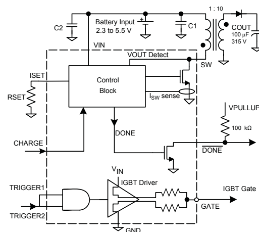
Figure 2. Typical application with single trigger input.
