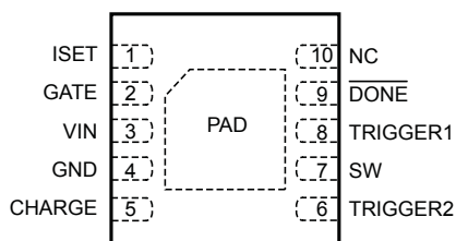
Pin-out Diagram
