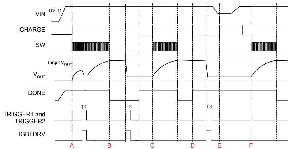
A8731 Operation Timing Diagram
