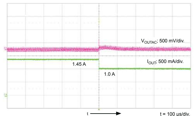
Detail: Step Down Transient Response
