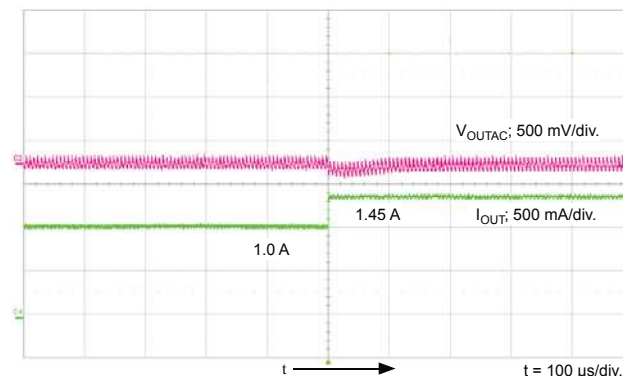
Detail: Step Up Transient Response
