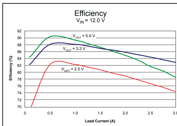
Efficiency curves for circuit at left.
