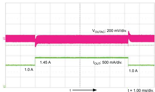
Transient Response
