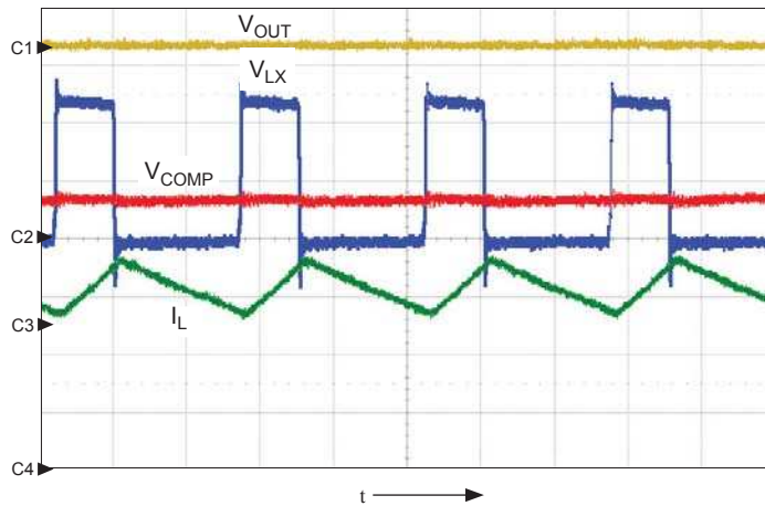
PWM at 3.3 A Load; shows V_{OUT} (ch1, 1 V/div.), V_{LX} (ch2, 5 V/div.), V_{COMP} (ch3, 500 mV/div.), I_L (ch4, 1 A/div.), t = 200 ns/div.
