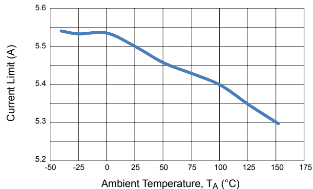
Switch Overcurrent Limit versus Temperature
