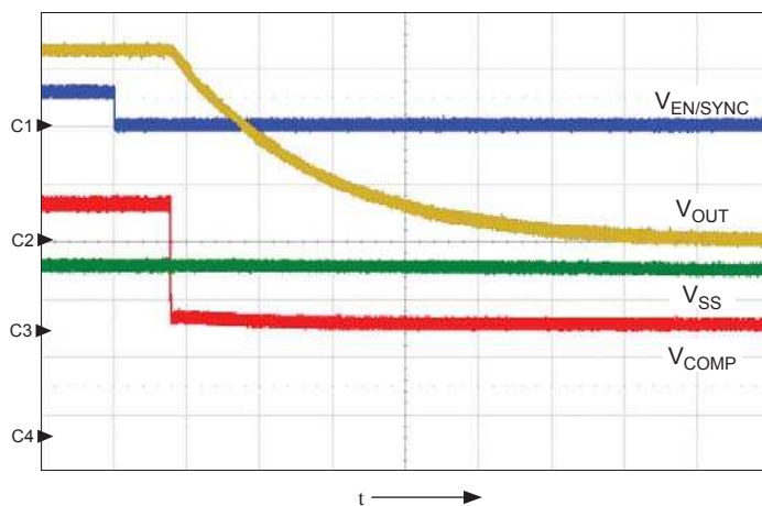
Shutdown at 3.3 A; shows V_{EN/SYNC} (ch1, 10 V/div.), V_{OUT} (ch2, 1 V/div.), V_{COMP} (ch3, 500 mV/div.), V_{SS} (ch3, 1 V/div.), t = 500 \mu s/div.
