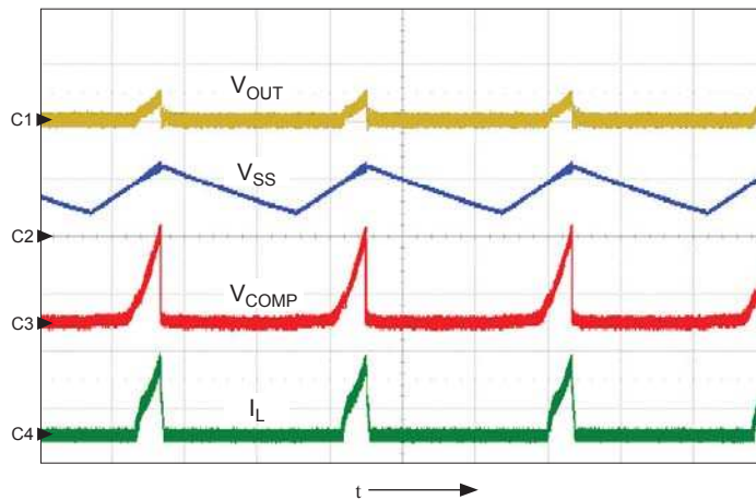
Hiccup Mode Operation; shows V_{OUT} (ch1, 1 V/div.), V_{SS} (ch2, 500 mV/div.), V_{COMP} (ch3, 1 V/div.), I_L (ch4, 5 A/div.), t = 500 \mu s/div.
