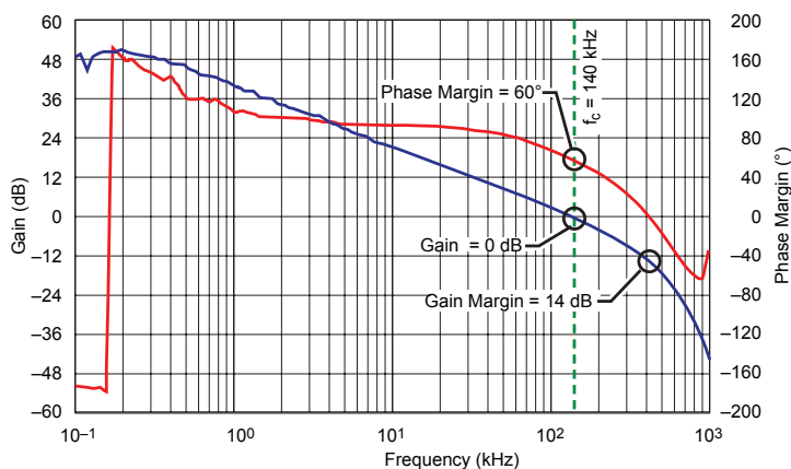
Bode Plot
