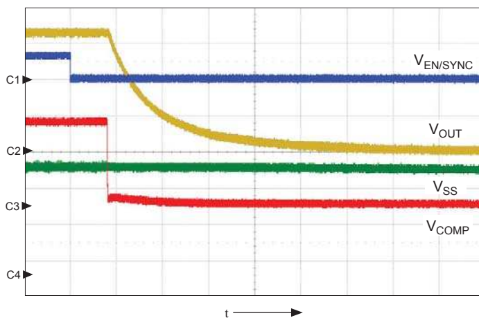
Shutdown at 2.2 A; shows V_{EN/SYNC} (ch1, 5 V/div.), V_{OUT} (ch2, 1 V/div.), V_{COMP} (ch3, 500 mV/div.), V_{SS} (ch4, 1 V/div.), t = 20 \mu s/div.
