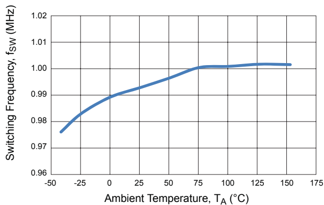
Switching Frequency versus Temperature
