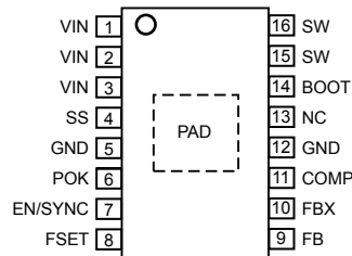
Pin-out Diagram
