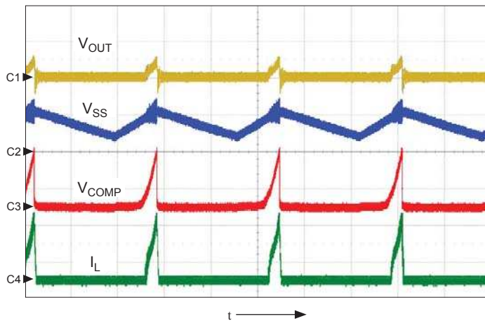
Hiccup Mode Operation; shows V_{OUT} (ch1, 500 mV/div.), V_{SS} (ch2, 500 mV/div.), V_{COMP} (ch3, 1 V/div.), I_L (ch4, 2 A/div.), t = 500 \mu s/div.
