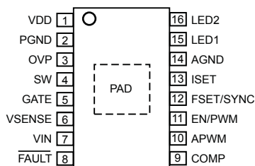
Pin-out Diagram
