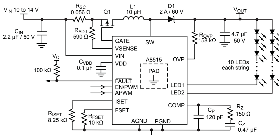
Figure 32. The schematic diagram showing calculated values from the design example above
