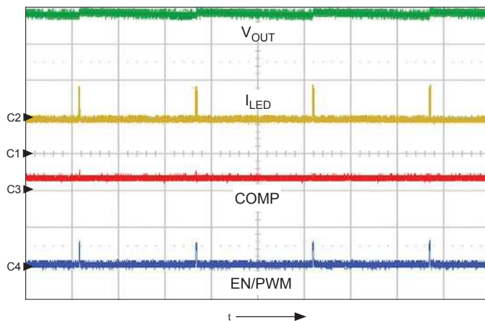
Figure 12B. Typical PWM diagram showing V_{OUT} , I_{LED} , and COMP pin as well as the PWM signal. PWM dimming frequency is 200 Hz at 1% duty cycle; shows V_{OUT} (ch1, 10 V/div.), I_{LED} (ch2, 50 mA/div.), COMP (ch3, 2 V/div.), EN/PWM (ch4, 5 V/div.), t = 2 ms/div.
