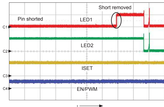
4B. Example with one LED shorted to GND. The IC will not proceed with power-up until the shorted LED pin is released, at which point the LED is checked to see if it is being used; shows LED1 (ch1, 500 mV/div.), LED2 (ch2, 500 mV/div.), ISET (ch3, 1 V/div.), and EN/PWM (ch4, 5 V/div.) pins, t = 1 ms/div .
