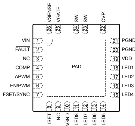
Pin-out Diagram
