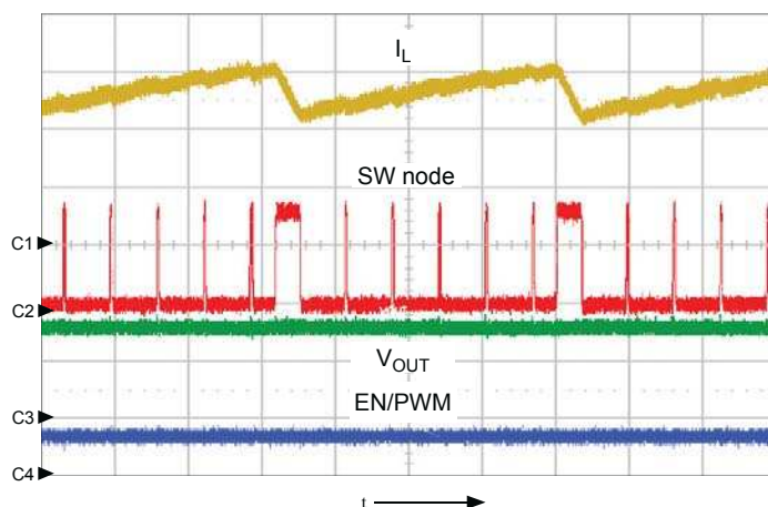
Figure 26. Cycle-by-cycle current limiting; inductor current ( I_L ), note reduction in output voltage as compared to normal operation with the same configuration (figure 25); shows I_L (ch1, 1 A/div.), SW node (ch2, 20 V/div.), V_{OUT} (ch3, 10 V/div.), and EN/PWM (ch4, 5 V/div.), t = 2 \mu\text{s}/\text{div.}
