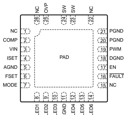
Pin-out Diagram
