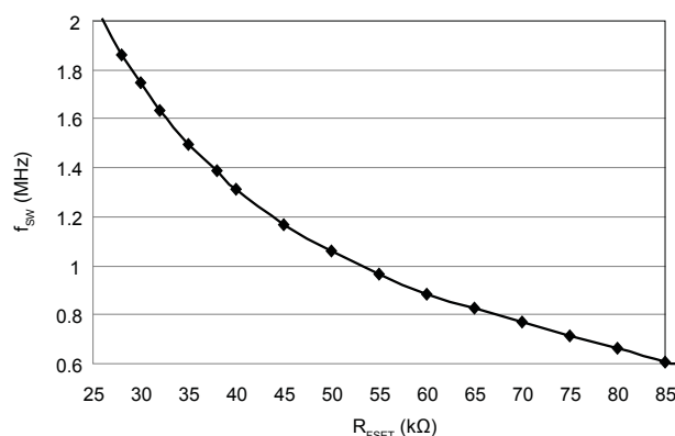
Figure 3. Switching frequency setting versus R_{FSET} ( V_{IN} = 5 V, V_{BAT} = 12 V).
