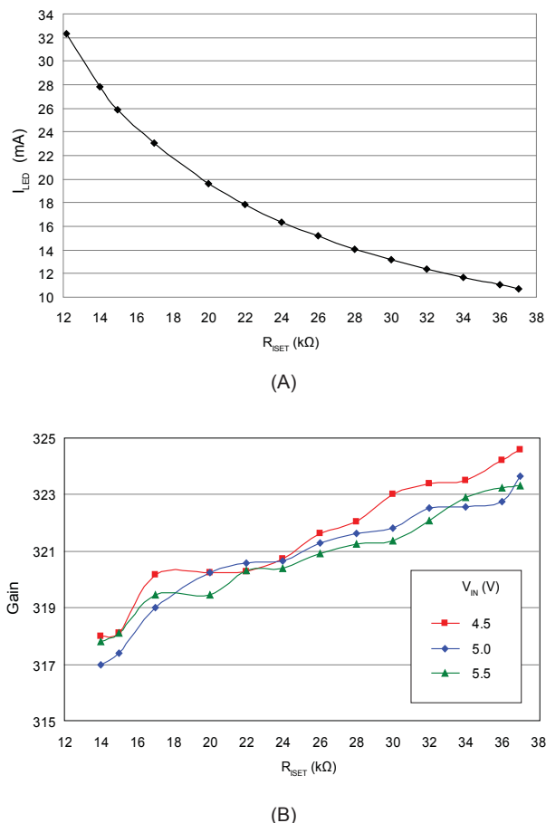
Figure 2. Effect of value of R_{ISET} on current through an LED string. Panel A shows level of 100% current, and panel B shows LEDx gain.
