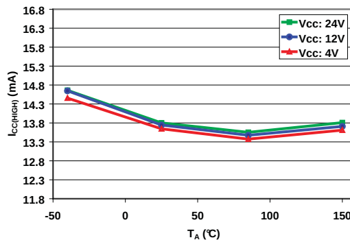
Supply Current (High) versus Ambient Temperature
